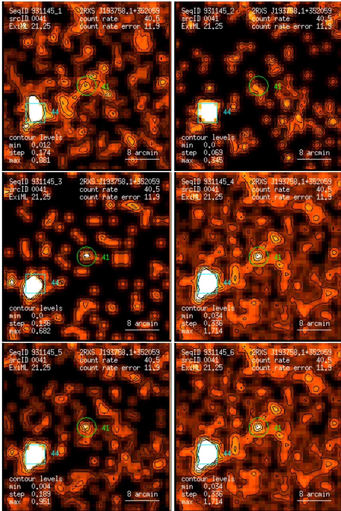
Figure 41: RASS 931145: detection 0041: band rate images, Gaussian filter: (1) PSPC channels 11 – 41, (2) 52 – 90, (3) 91 – 201, (4) 11 – 235, (5) 52 – 201, (6) 11 – 201. Broad band rates in counts/ks. Band rate contour levels in counts/ks/arcmin 2 .
