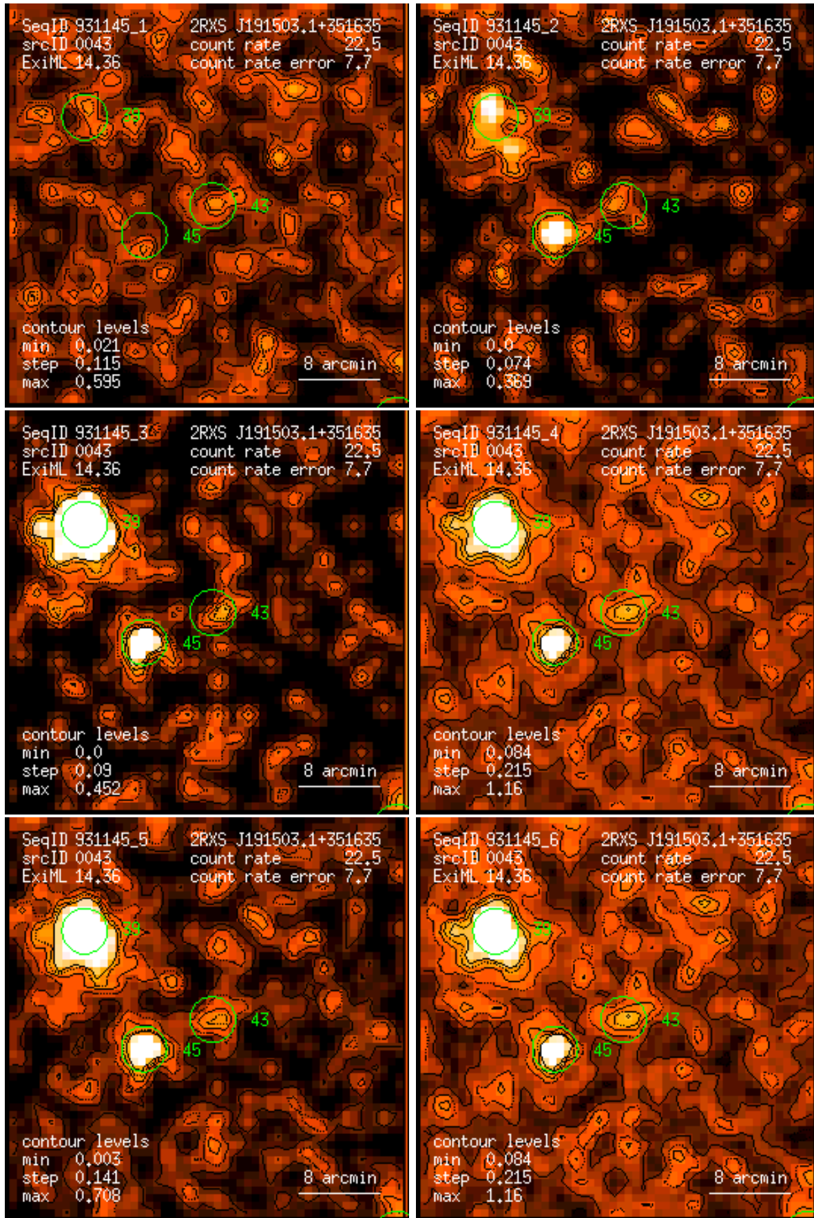
Figure 43: RASS 931145: detection 0043: band rate images, Gaussian filter: (1) PSPC channels 11 – 41, (2) 52 – 90, (3) 91 – 201, (4) 11 – 235, (5) 52 – 201, (6) 11 – 201. Broad band rates in counts/ks. Band rate contour levels in counts/ks/arcmin 2 .
