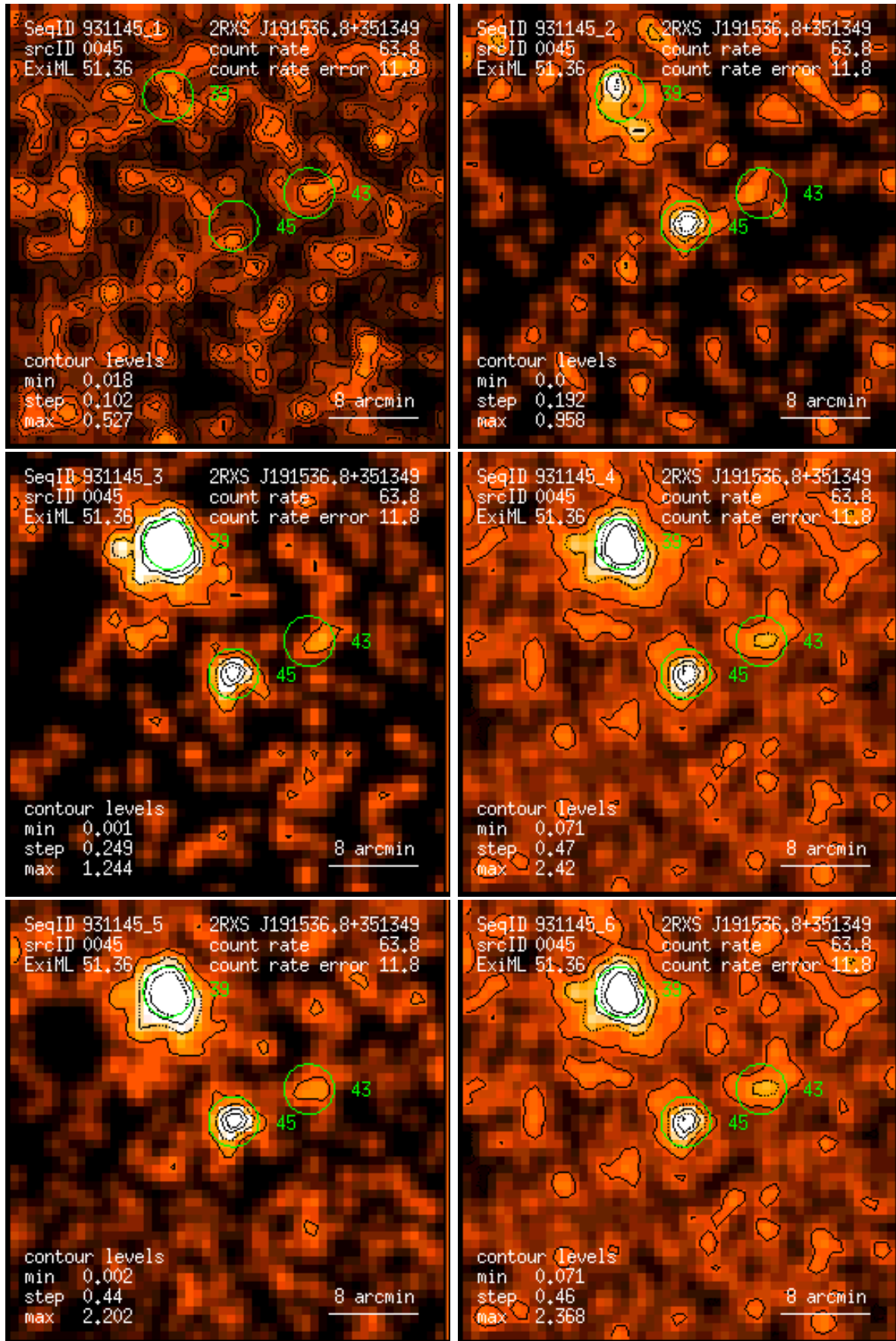
Figure 45: RASS 931145: detection 0045: band rate images, Gaussian filter: (1) PSPC channels 11 – 41, (2) 52 – 90, (3) 91 – 201, (4) 11 – 235, (5) 52 – 201, (6) 11 – 201. Broad band rates in counts/ks. Band rate contour levels in counts/ks/arcmin 2 .
