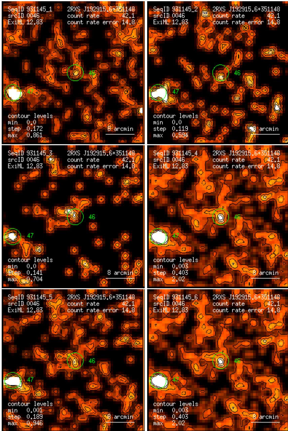
Figure 46: RASS 931145: detection 0046: band rate images, Gaussian filter: (1) PSPC channels 11 – 41, (2) 52 – 90, (3) 91 – 201, (4) 11 – 235, (5) 52 – 201, (6) 11 – 201. Broad band rates in counts/ks. Band rate contour levels in counts/ks/arcmin 2 .
