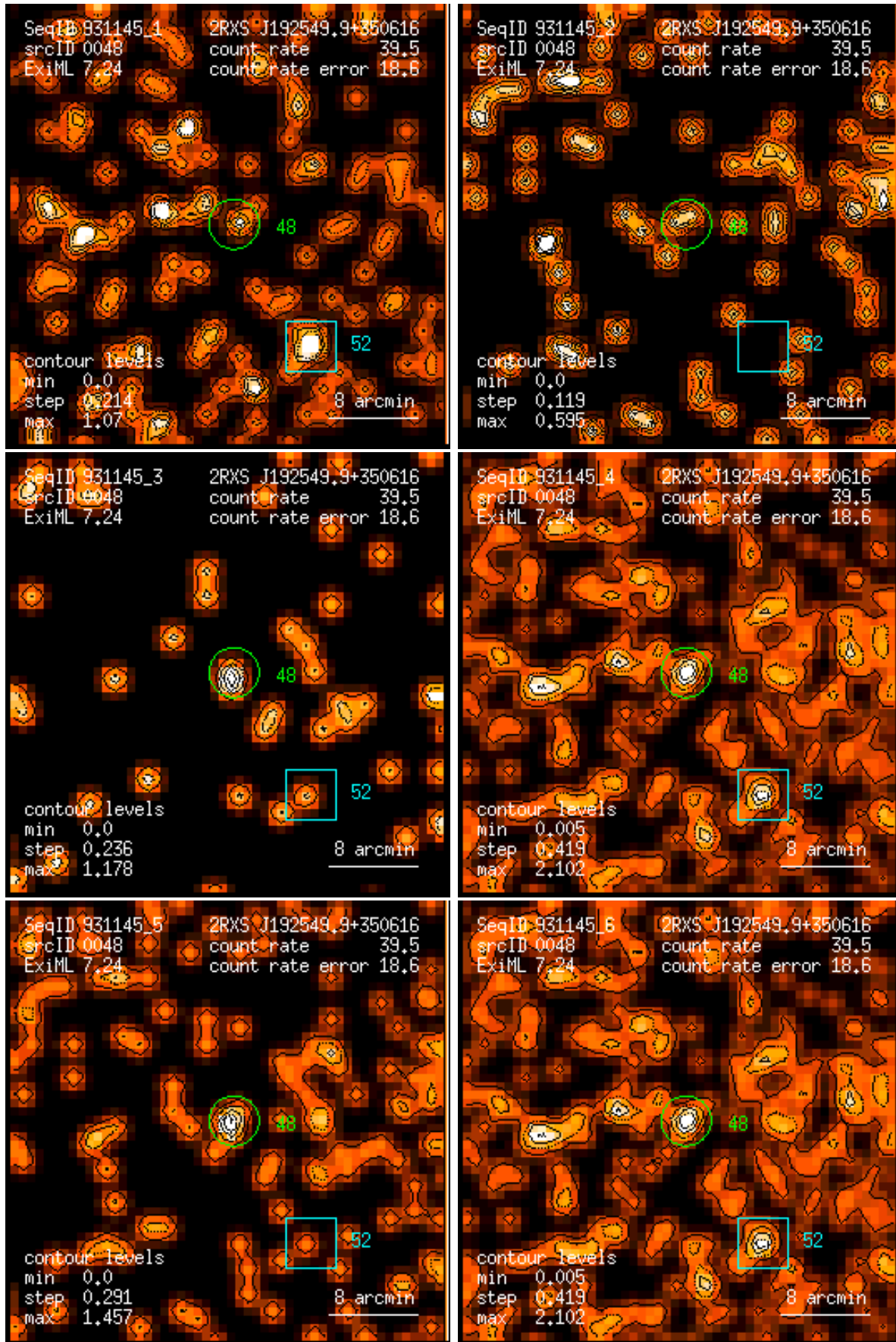
Figure 48: RASS 931145: detection 0048: band rate images, Gaussian filter: (1) PSPC channels 11 – 41, (2) 52 – 90, (3) 91 – 201, (4) 11 – 235, (5) 52 – 201, (6) 11 – 201. Broad band rates in counts/ks. Band rate contour levels in counts/ks/arcmin 2 .
