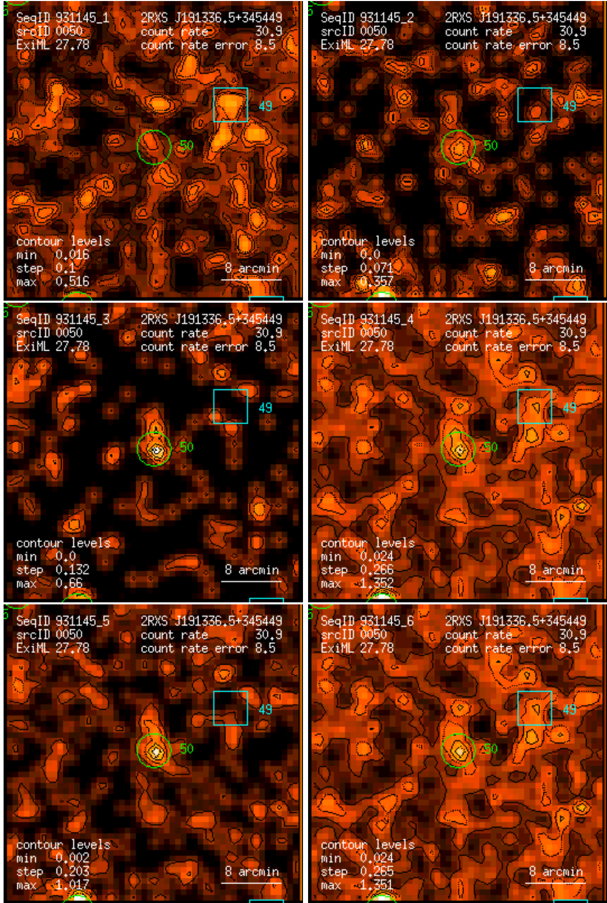
Figure 50: RASS 931145: detection 0050: band rate images, Gaussian filter: (1) PSPC channels 11 – 41, (2) 52 – 90, (3) 91 – 201, (4) 11 – 235, (5) 52 – 201, (6) 11 – 201. Broad band rates in counts/ks. Band rate contour levels in counts/ks/arcmin 2 .
