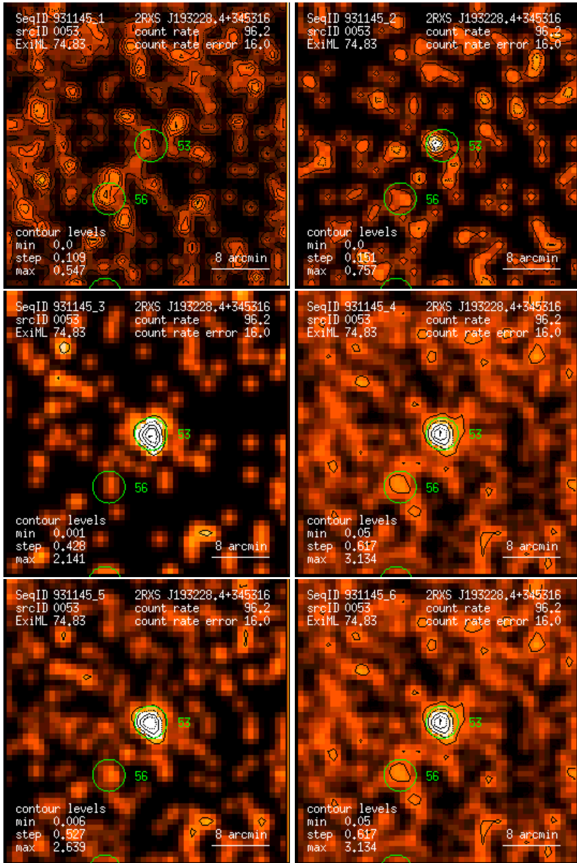
Figure 53: RASS 931145: detection 0053: band rate images, Gaussian filter: (1) PSPC channels 11 – 41, (2) 52 – 90, (3) 91 – 201, (4) 11 – 235, (5) 52 – 201, (6) 11 – 201. Broad band rates in counts/ks. Band rate contour levels in counts/ks/arcmin 2 .
