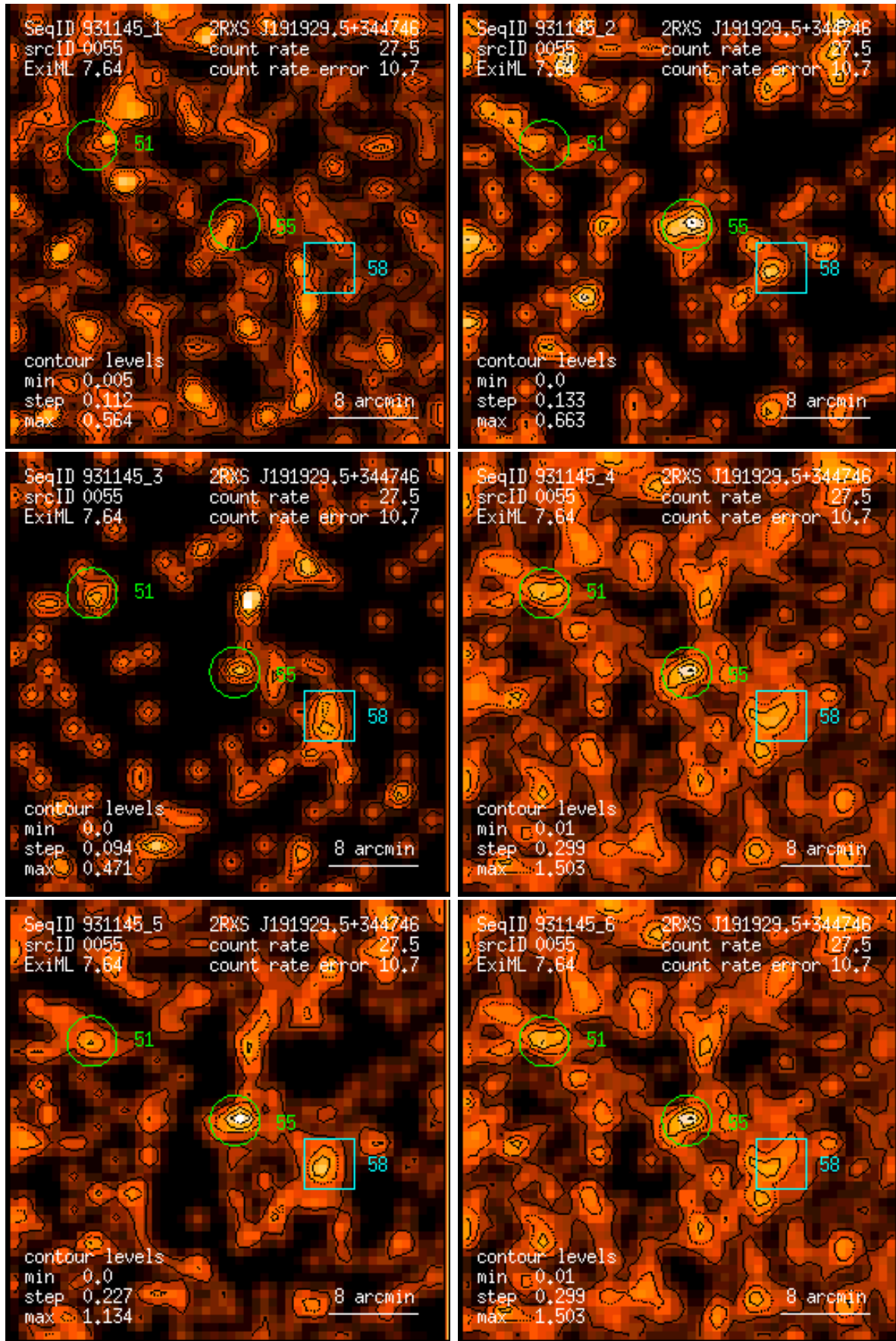
Figure 55: RASS 931145: detection 0055: band rate images, Gaussian filter: (1) PSPC channels 11 – 41, (2) 52 – 90, (3) 91 – 201, (4) 11 – 235, (5) 52 – 201, (6) 11 – 201. Broad band rates in counts/ks. Band rate contour levels in counts/ks/arcmin 2 .
