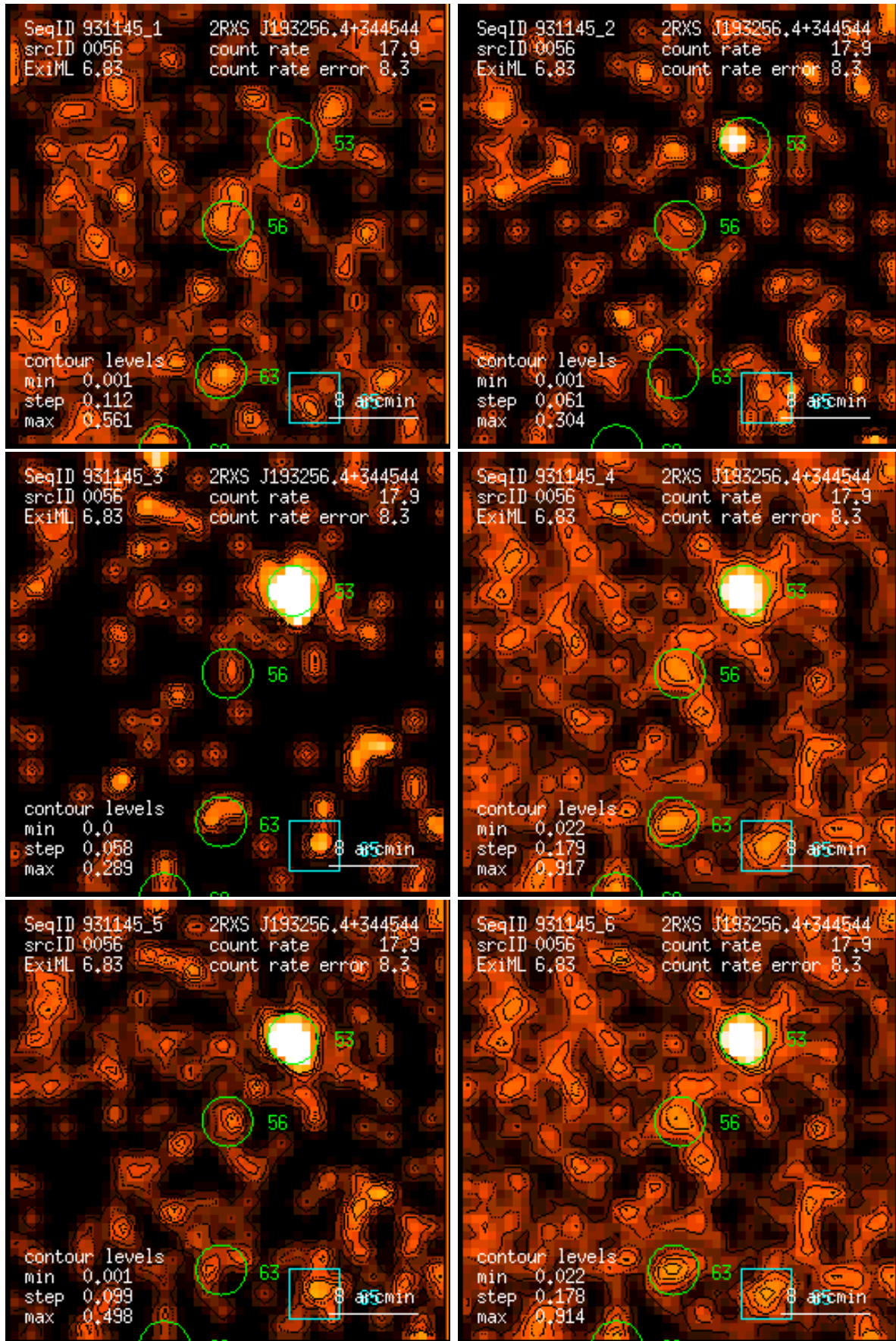
Figure 56: RASS 931145: detection 0056: band rate images, Gaussian filter: (1) PSPC channels 11 – 41, (2) 52 – 90, (3) 91 – 201, (4) 11 – 235, (5) 52 – 201, (6) 11 – 201. Broad band rates in counts/ks. Band rate contour levels in counts/ks/arcmin 2 .
