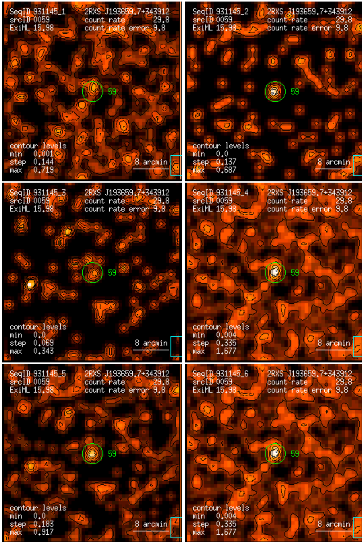
Figure 59: RASS 931145: detection 0059: band rate images, Gaussian filter: (1) PSPC channels 11 – 41, (2) 52 – 90, (3) 91 – 201, (4) 11 – 235, (5) 52 – 201, (6) 11 – 201. Broad band rates in counts/ks. Band rate contour levels in counts/ks/arcmin 2 .
