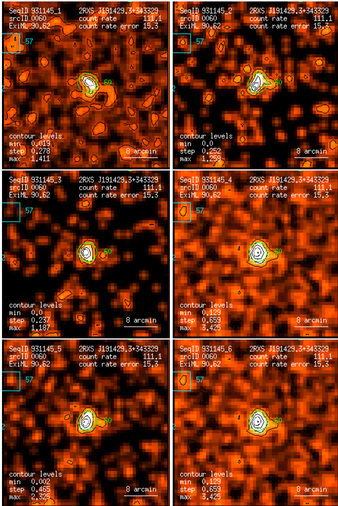
Figure 60: RASS 931145: detection 0060: band rate images, Gaussian filter: (1) PSPC channels 11 – 41, (2) 52 – 90, (3) 91 – 201, (4) 11 – 235, (5) 52 – 201, (6) 11 – 201. Broad band rates in counts/ks. Band rate contour levels in counts/ks/arcmin 2 .
