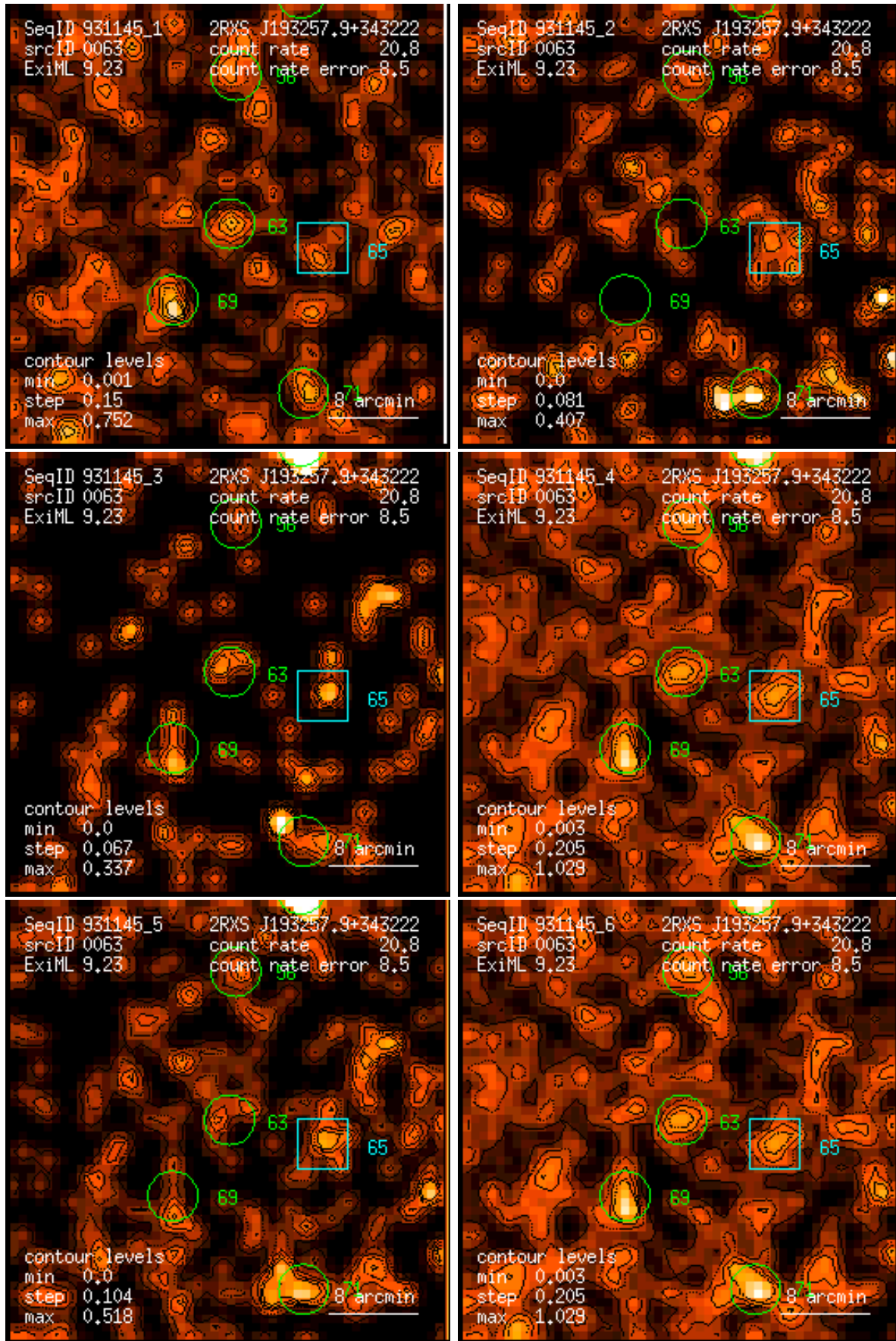
Figure 63: RASS 931145: detection 0063: band rate images, Gaussian filter: (1) PSPC channels 11 – 41, (2) 52 – 90, (3) 91 – 201, (4) 11 – 235, (5) 52 – 201, (6) 11 – 201. Broad band rates in counts/ks. Band rate contour levels in counts/ks/arcmin 2 .
