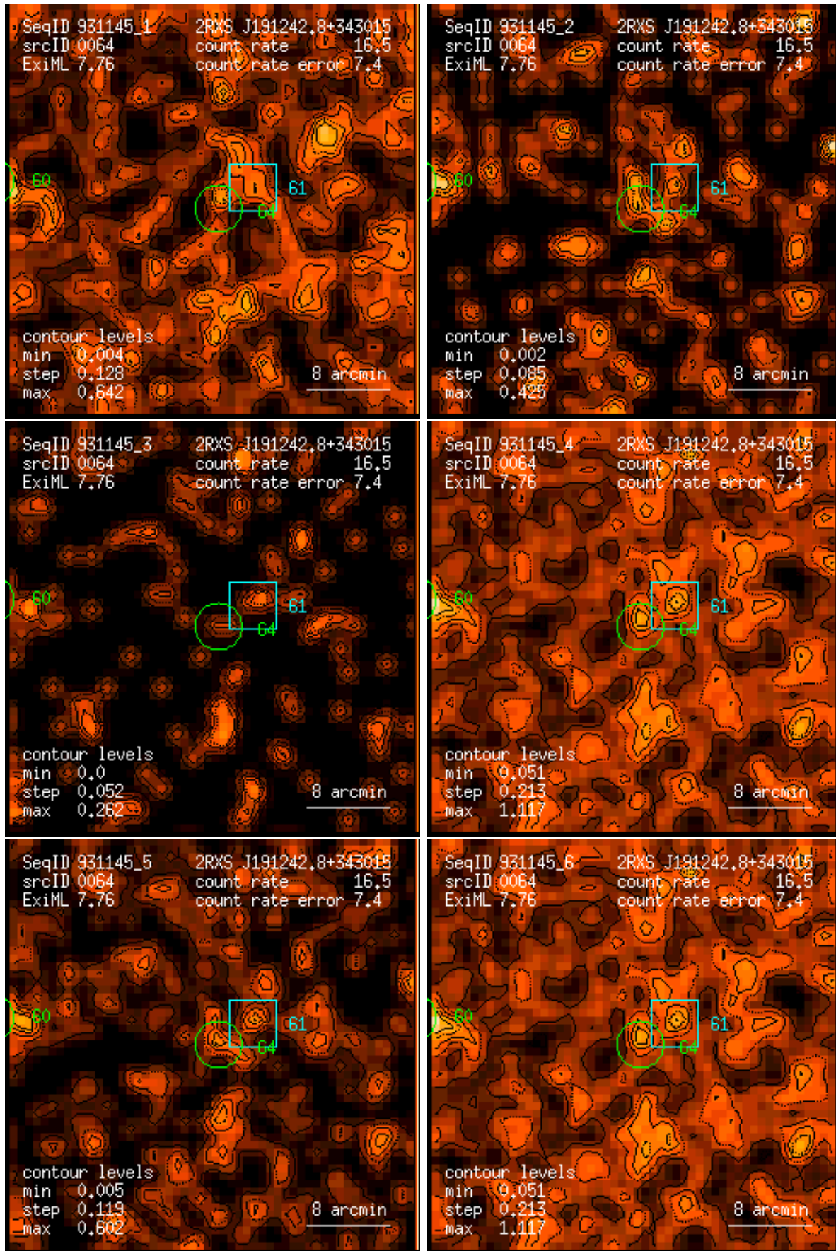
Figure 64: RASS 931145: detection 0064: band rate images, Gaussian filter: (1) PSPC channels 11 – 41, (2) 52 – 90, (3) 91 – 201, (4) 11 – 235, (5) 52 – 201, (6) 11 – 201. Broad band rates in counts/ks. Band rate contour levels in counts/ks/arcmin 2 .
