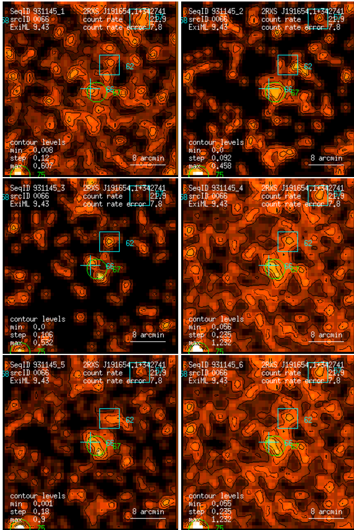
Figure 66: RASS 931145: detection 0066: band rate images, Gaussian filter: (1) PSPC channels 11 – 41, (2) 52 – 90, (3) 91 – 201, (4) 11 – 235, (5) 52 – 201, (6) 11 – 201. Broad band rates in counts/ks. Band rate contour levels in counts/ks/arcmin 2 .
