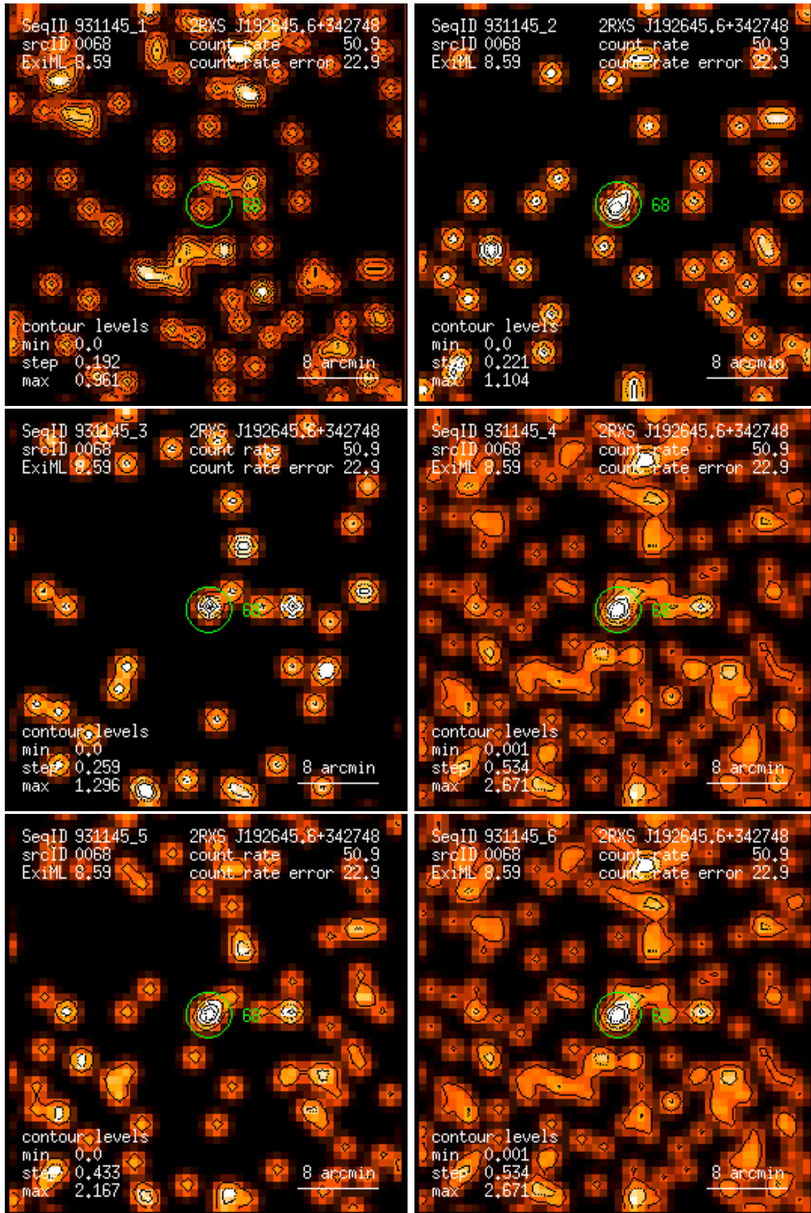
Figure 68: RASS 931145: detection 0068: band rate images, Gaussian filter: (1) PSPC channels 11 – 41, (2) 52 – 90, (3) 91 – 201, (4) 11 – 235, (5) 52 – 201, (6) 11 – 201. Broad band rates in counts/ks. Band rate contour levels in counts/ks/arcmin 2 .
