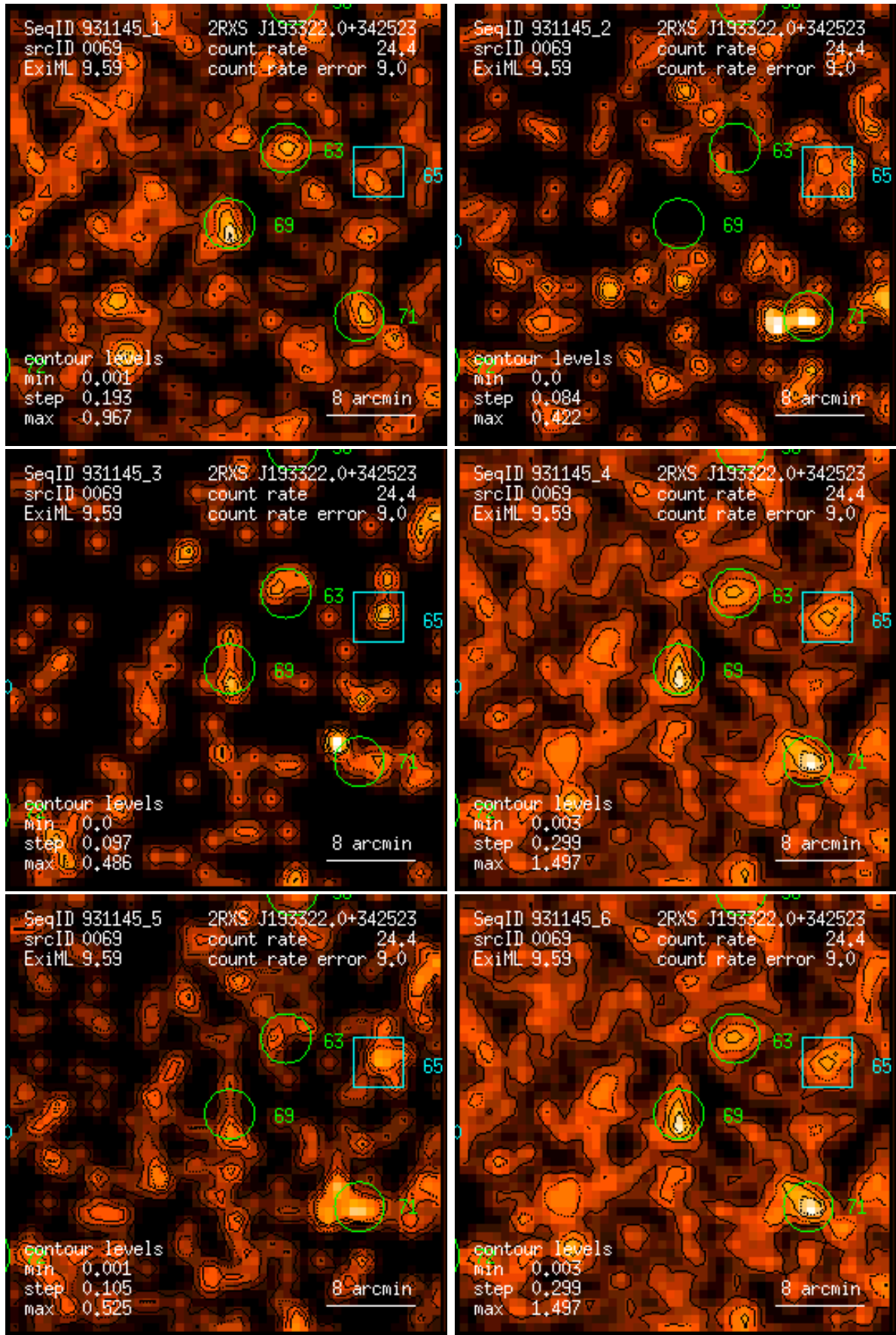
Figure 69: RASS 931145: detection 0069: band rate images, Gaussian filter: (1) PSPC channels 11 – 41, (2) 52 – 90, (3) 91 – 201, (4) 11 – 235, (5) 52 – 201, (6) 11 – 201. Broad band rates in counts/ks. Band rate contour levels in counts/ks/arcmin 2 .
