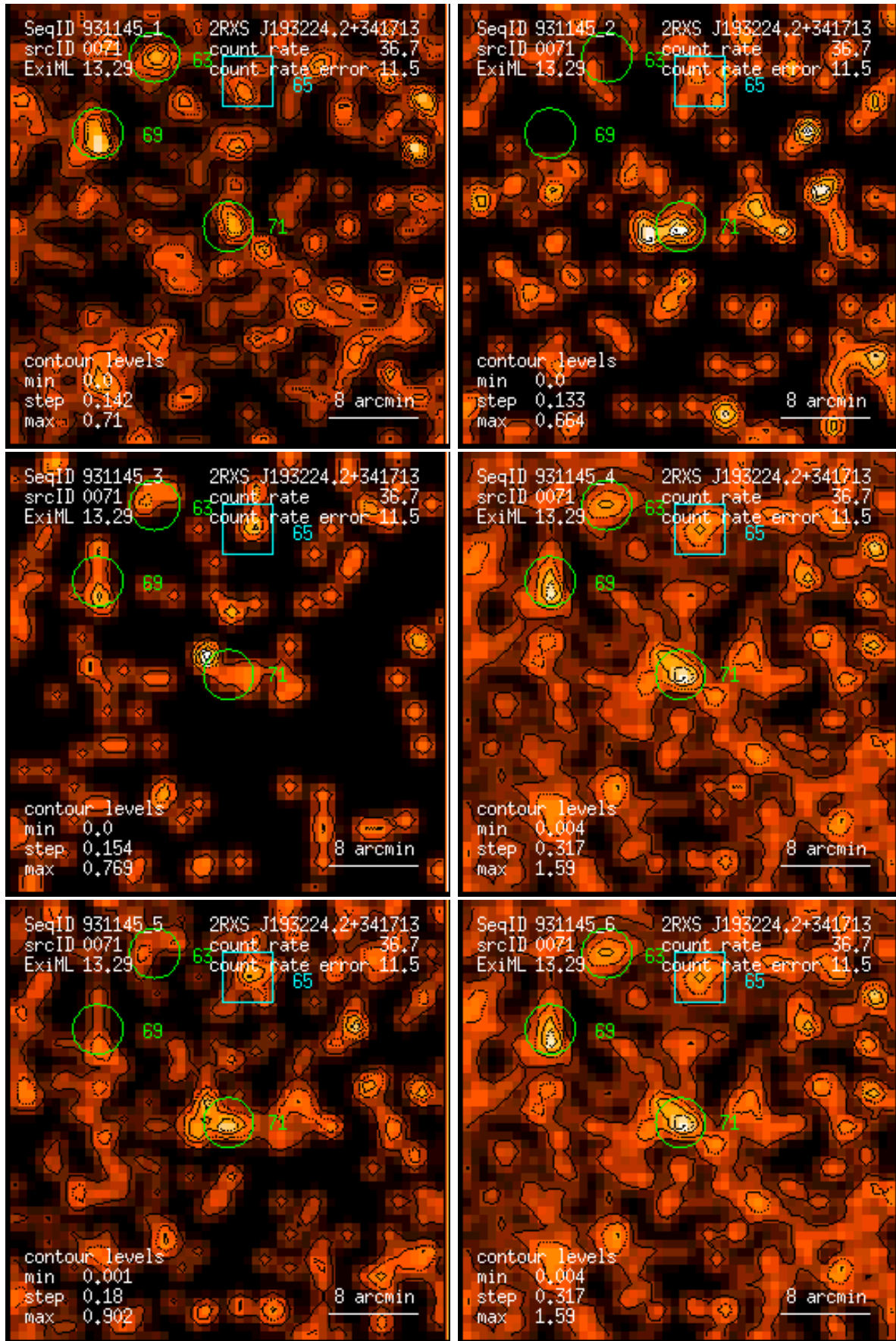
Figure 71: RASS 931145: detection 0071: band rate images, Gaussian filter: (1) PSPC channels 11 – 41, (2) 52 – 90, (3) 91 – 201, (4) 11 – 235, (5) 52 – 201, (6) 11 – 201. Broad band rates in counts/ks. Band rate contour levels in counts/ks/arcmin 2 .
