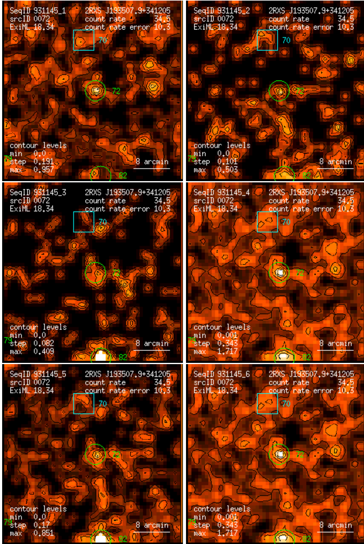
Figure 72: RASS 931145: detection 0072: band rate images, Gaussian filter: (1) PSPC channels 11 – 41, (2) 52 – 90, (3) 91 – 201, (4) 11 – 235, (5) 52 – 201, (6) 11 – 201. Broad band rates in counts/ks. Band rate contour levels in counts/ks/arcmin 2 .
