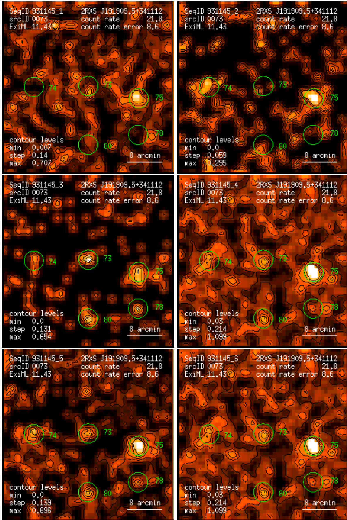
Figure 73: RASS 931145: detection 0073: band rate images, Gaussian filter: (1) PSPC channels 11 – 41, (2) 52 – 90, (3) 91 – 201, (4) 11 – 235, (5) 52 – 201, (6) 11 – 201. Broad band rates in counts/ks. Band rate contour levels in counts/ks/arcmin 2 .
