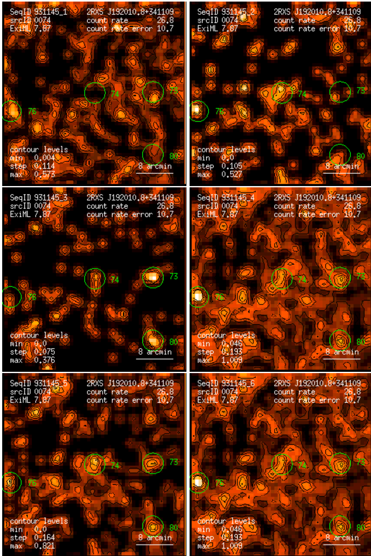
Figure 74: RASS 931145: detection 0074: band rate images, Gaussian filter: (1) PSPC channels 11 – 41, (2) 52 – 90, (3) 91 – 201, (4) 11 – 235, (5) 52 – 201, (6) 11 – 201. Broad band rates in counts/ks. Band rate contour levels in counts/ks/arcmin 2 .
