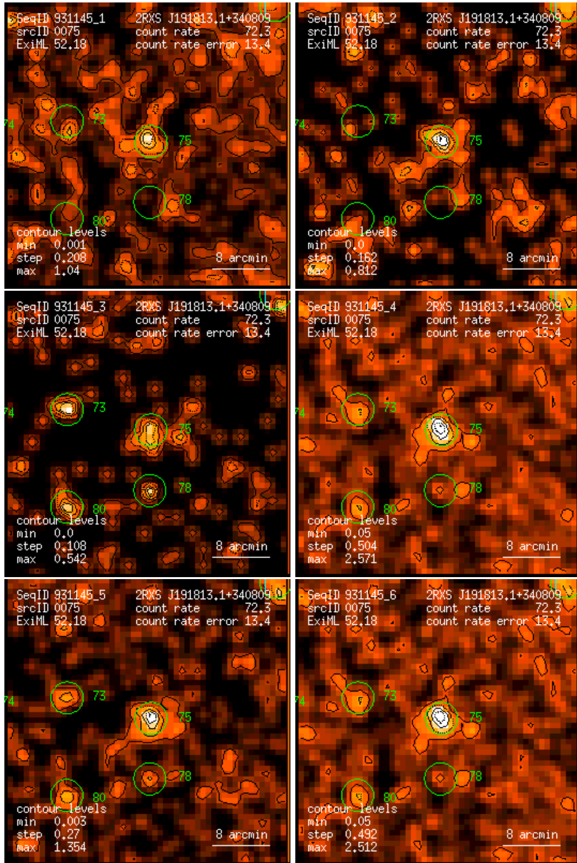
Figure 75: RASS 931145: detection 0075: band rate images, Gaussian filter: (1) PSPC channels 11 – 41, (2) 52 – 90, (3) 91 – 201, (4) 11 – 235, (5) 52 – 201, (6) 11 – 201. Broad band rates in counts/ks. Band rate contour levels in counts/ks/arcmin 2 .
