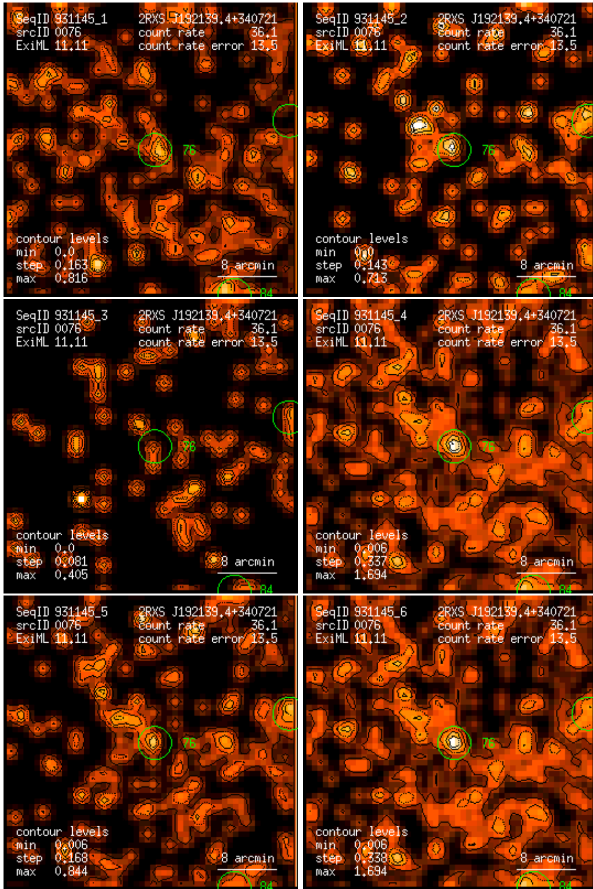
Figure 76: RASS 931145: detection 0076: band rate images, Gaussian filter: (1) PSPC channels 11 – 41, (2) 52 – 90, (3) 91 – 201, (4) 11 – 235, (5) 52 – 201, (6) 11 – 201. Broad band rates in counts/ks. Band rate contour levels in counts/ks/arcmin 2 .
