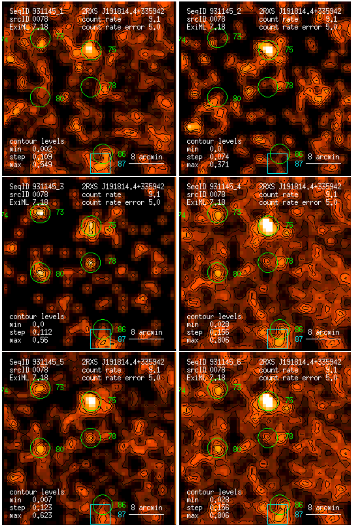
Figure 78: RASS 931145: detection 0078: band rate images, Gaussian filter: (1) PSPC channels 11 – 41, (2) 52 – 90, (3) 91 – 201, (4) 11 – 235, (5) 52 – 201, (6) 11 – 201. Broad band rates in counts/ks. Band rate contour levels in counts/ks/arcmin 2 .
