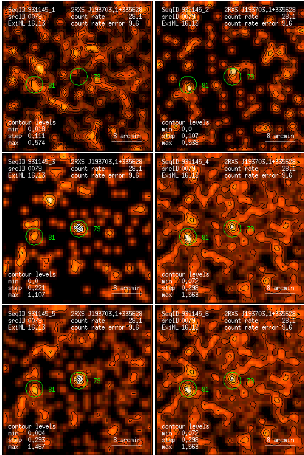
Figure 79: RASS 931145: detection 0079: band rate images, Gaussian filter: (1) PSPC channels 11 – 41, (2) 52 – 90, (3) 91 – 201, (4) 11 – 235, (5) 52 – 201, (6) 11 – 201. Broad band rates in counts/ks. Band rate contour levels in counts/ks/arcmin 2 .
