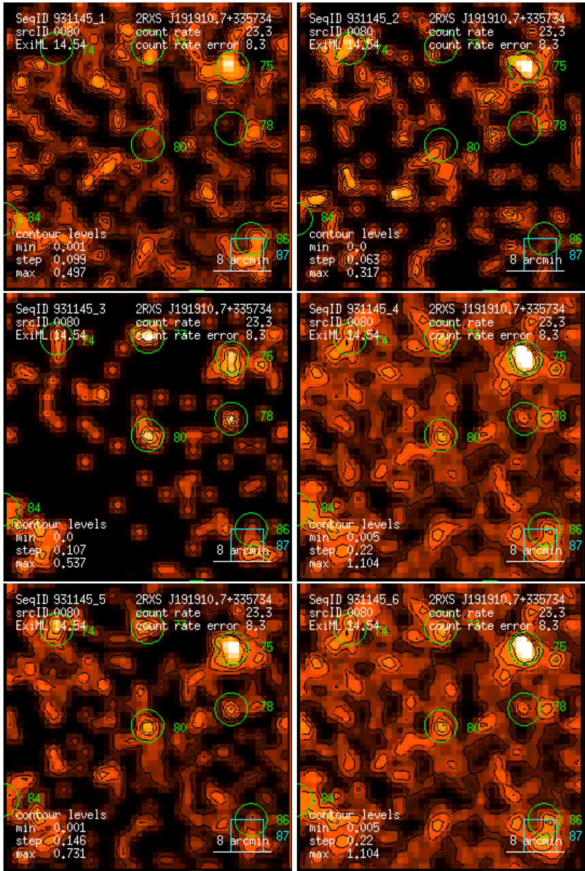
Figure 80: RASS 931145: detection 0080: band rate images, Gaussian filter: (1) PSPC channels 11 – 41, (2) 52 – 90, (3) 91 – 201, (4) 11 – 235, (5) 52 – 201, (6) 11 – 201. Broad band rates in counts/ks. Band rate contour levels in counts/ks/arcmin 2 .
