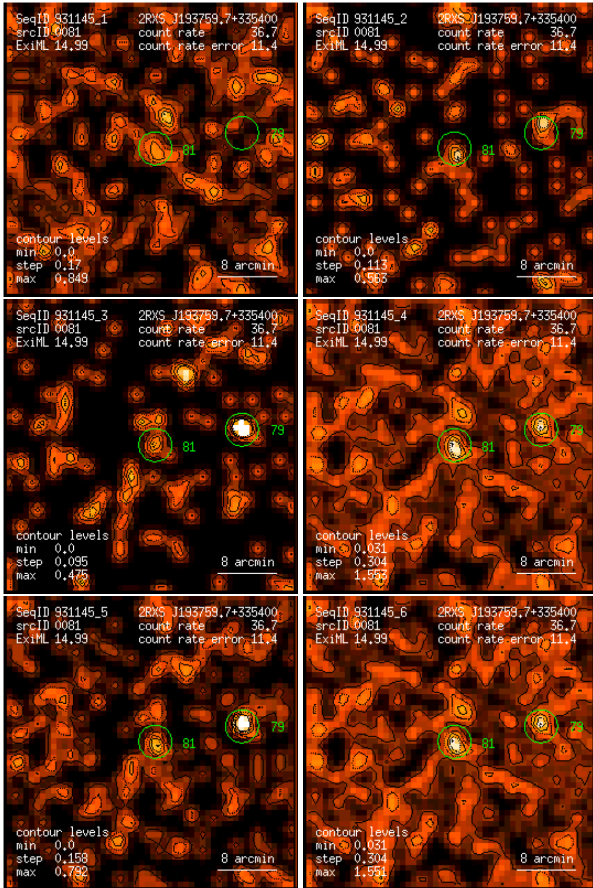
Figure 81: RASS 931145: detection 0081: band rate images, Gaussian filter: (1) PSPC channels 11 – 41, (2) 52 – 90, (3) 91 – 201, (4) 11 – 235, (5) 52 – 201, (6) 11 – 201. Broad band rates in counts/ks. Band rate contour levels in counts/ks/arcmin 2 .
