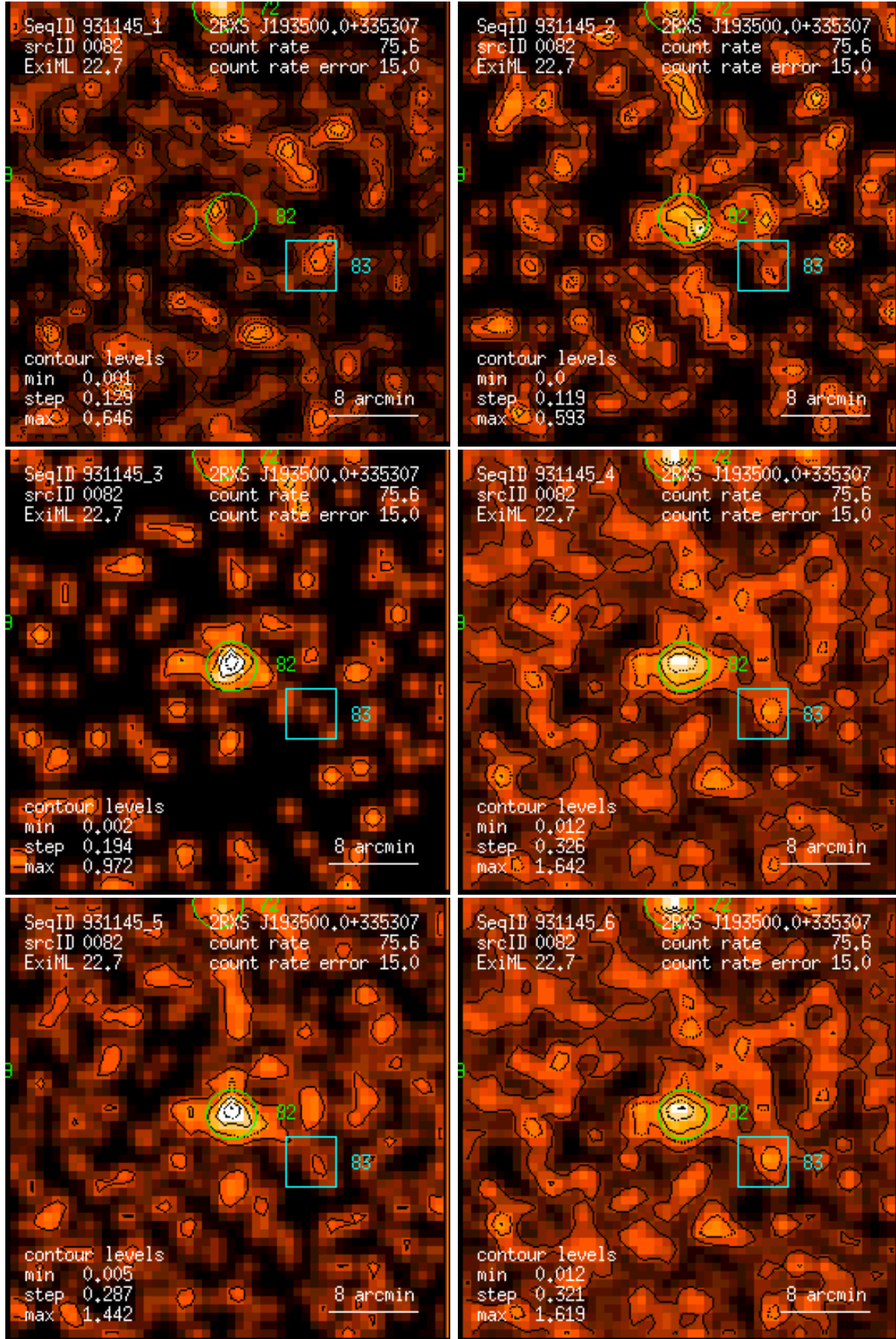
Figure 82: RASS 931145: detection 0082: band rate images, Gaussian filter: (1) PSPC channels 11 – 41, (2) 52 – 90, (3) 91 – 201, (4) 11 – 235, (5) 52 – 201, (6) 11 – 201. Broad band rates in counts/ks. Band rate contour levels in counts/ks/arcmin 2 .
