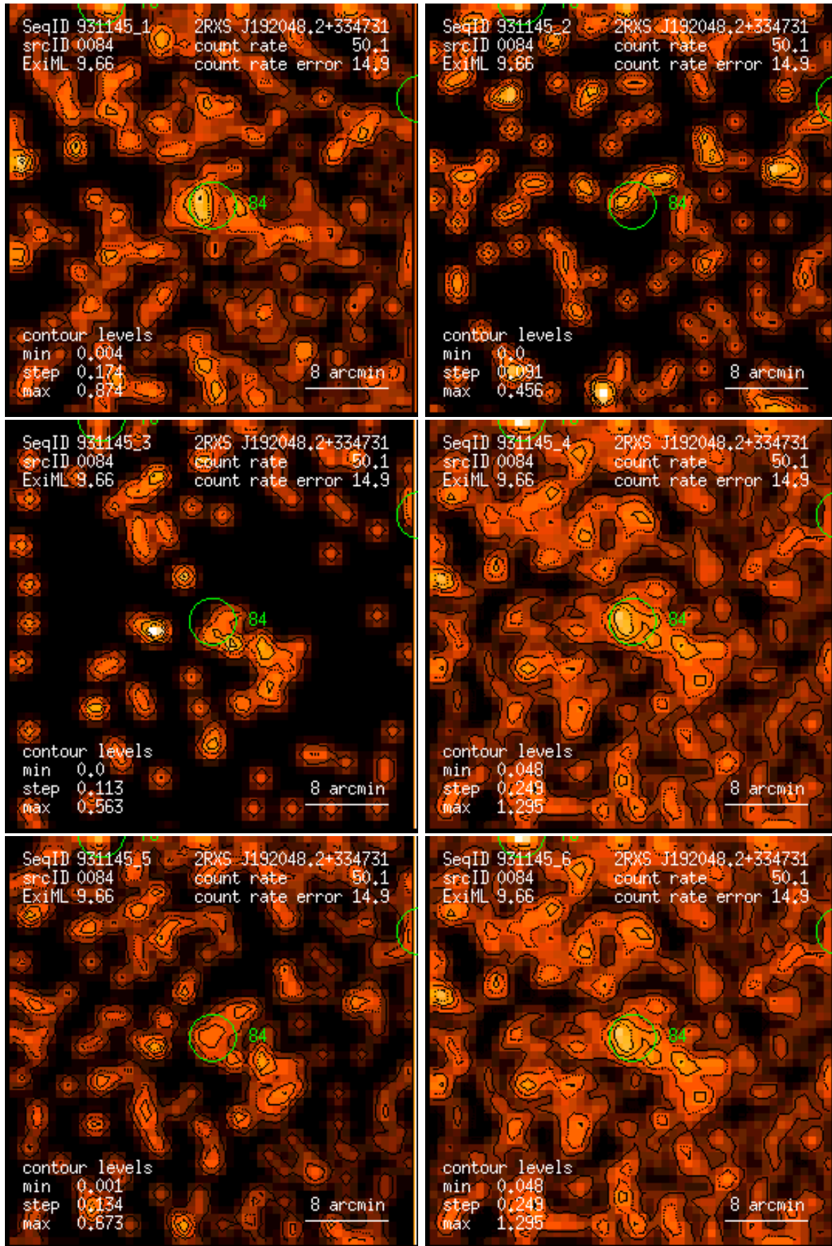
Figure 84: RASS 931145: detection 0084: band rate images, Gaussian filter: (1) PSPC channels 11 – 41, (2) 52 – 90, (3) 91 – 201, (4) 11 – 235, (5) 52 – 201, (6) 11 – 201. Broad band rates in counts/ks. Band rate contour levels in counts/ks/arcmin 2 .
