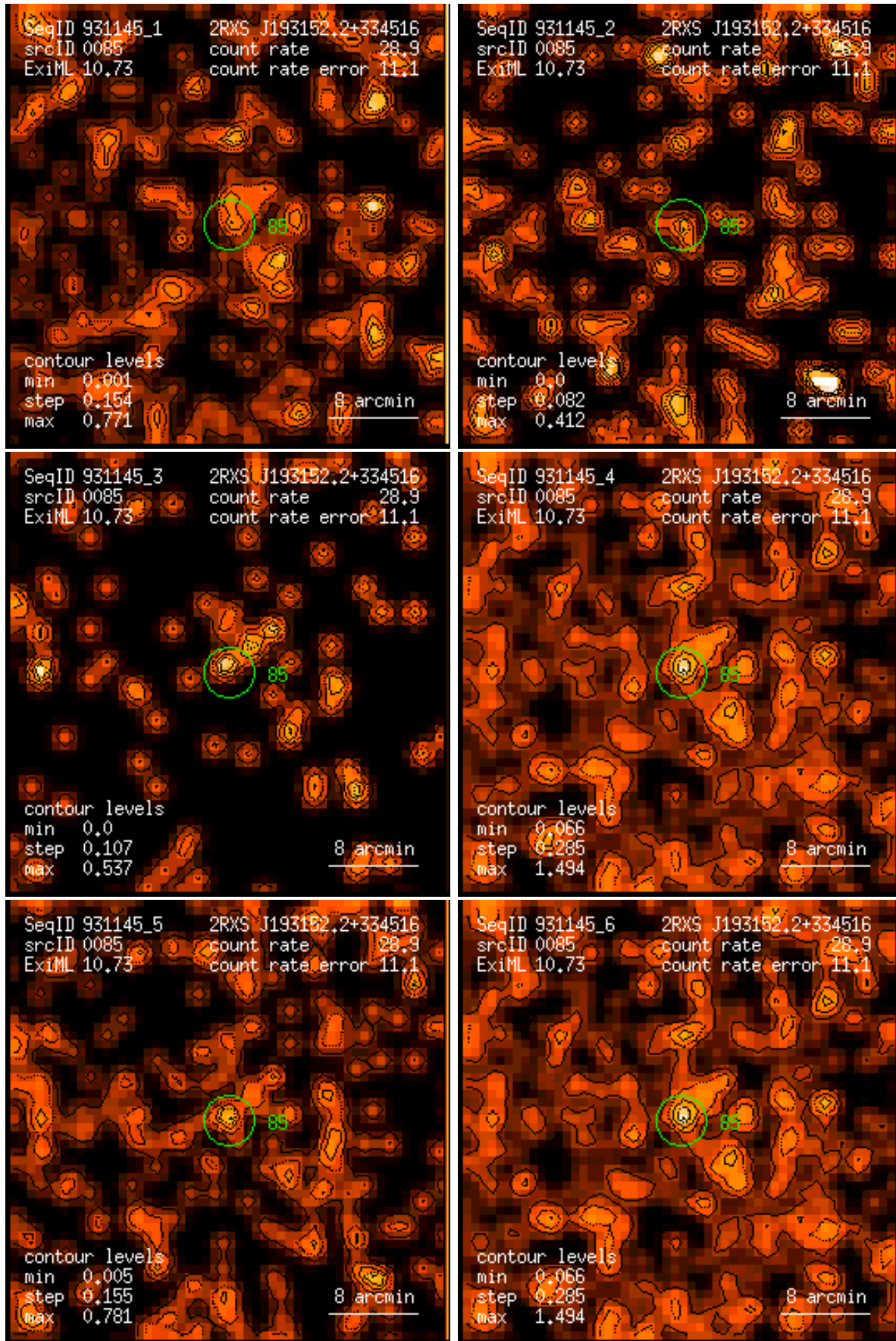
Figure 85: RASS 931145: detection 0085: band rate images, Gaussian filter: (1) PSPC channels 11 – 41, (2) 52 – 90, (3) 91 – 201, (4) 11 – 235, (5) 52 – 201, (6) 11 – 201. Broad band rates in counts/ks. Band rate contour levels in counts/ks/arcmin 2 .
