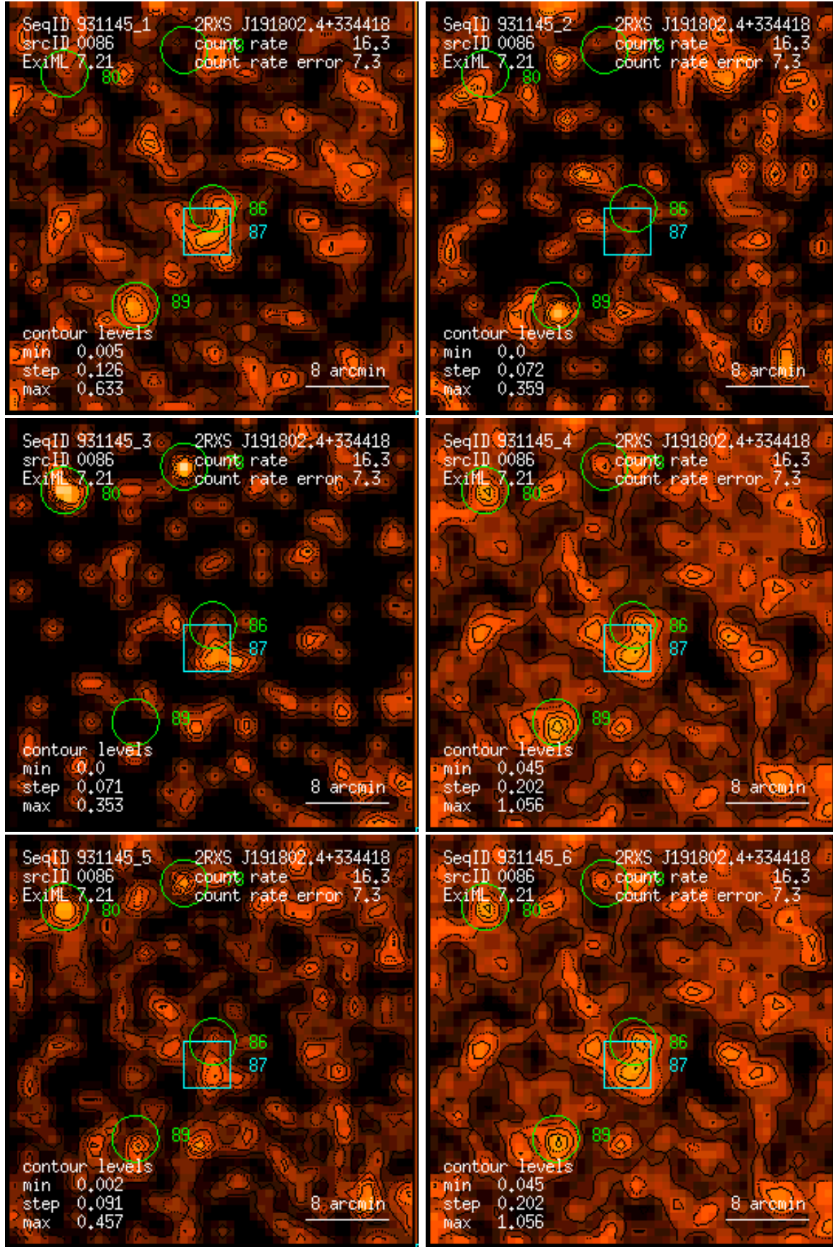
Figure 86: RASS 931145: detection 0086: band rate images, Gaussian filter: (1) PSPC channels 11 – 41, (2) 52 – 90, (3) 91 – 201, (4) 11 – 235, (5) 52 – 201, (6) 11 – 201. Broad band rates in counts/ks. Band rate contour levels in counts/ks/arcmin 2 .
