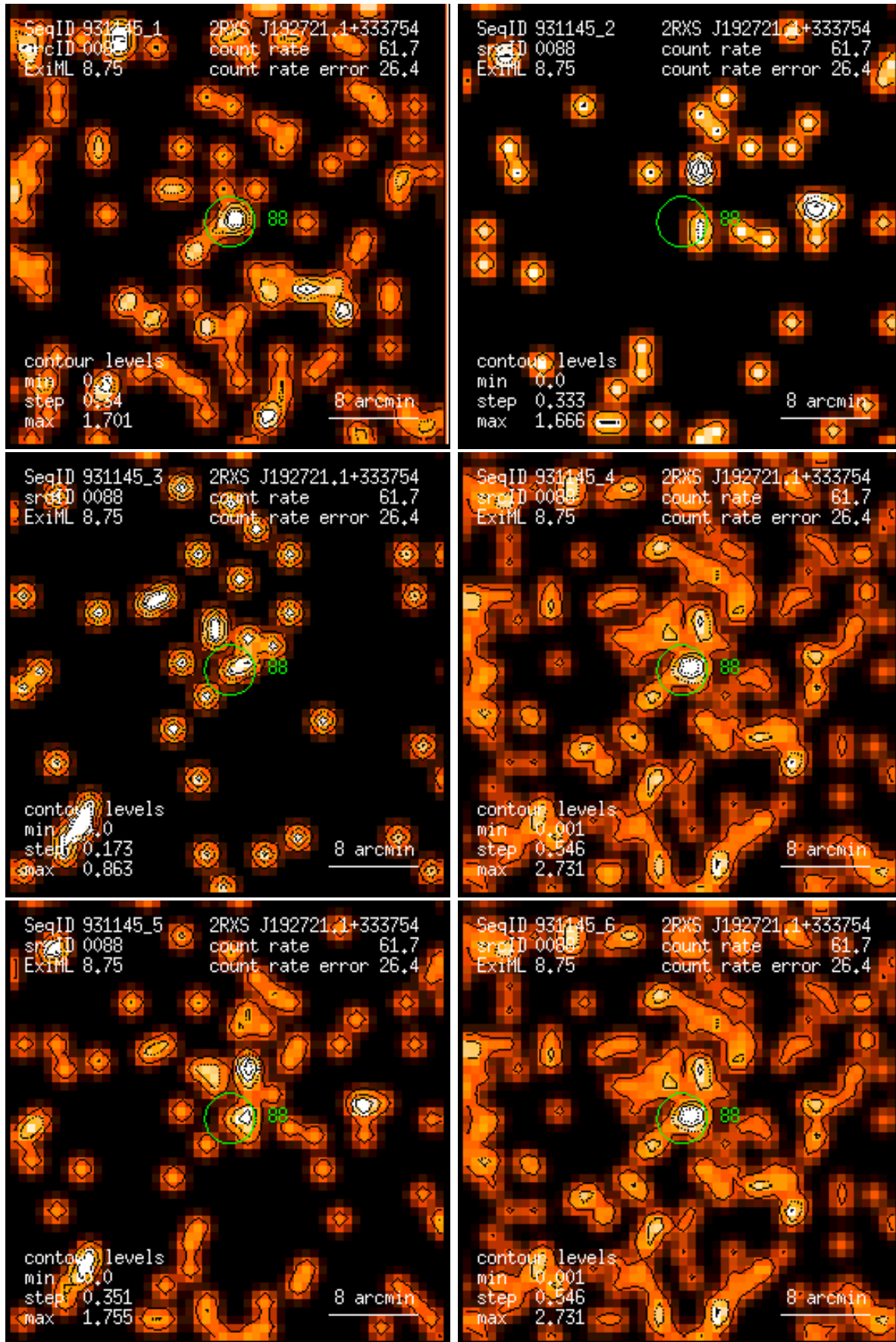
Figure 88: RASS 931145: detection 0088: band rate images, Gaussian filter: (1) PSPC channels 11 – 41, (2) 52 – 90, (3) 91 – 201, (4) 11 – 235, (5) 52 – 201, (6) 11 – 201. Broad band rates in counts/ks. Band rate contour levels in counts/ks/arcmin 2 .
