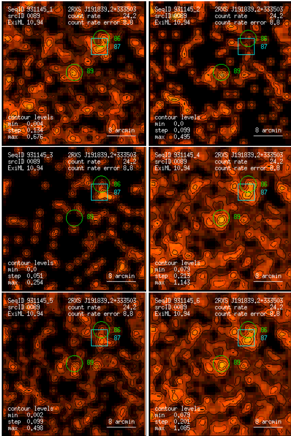
Figure 89: RASS 931145: detection 0089: band rate images, Gaussian filter: (1) PSPC channels 11 – 41, (2) 52 – 90, (3) 91 – 201, (4) 11 – 235, (5) 52 – 201, (6) 11 – 201. Broad band rates in counts/ks. Band rate contour levels in counts/ks/arcmin 2 .
