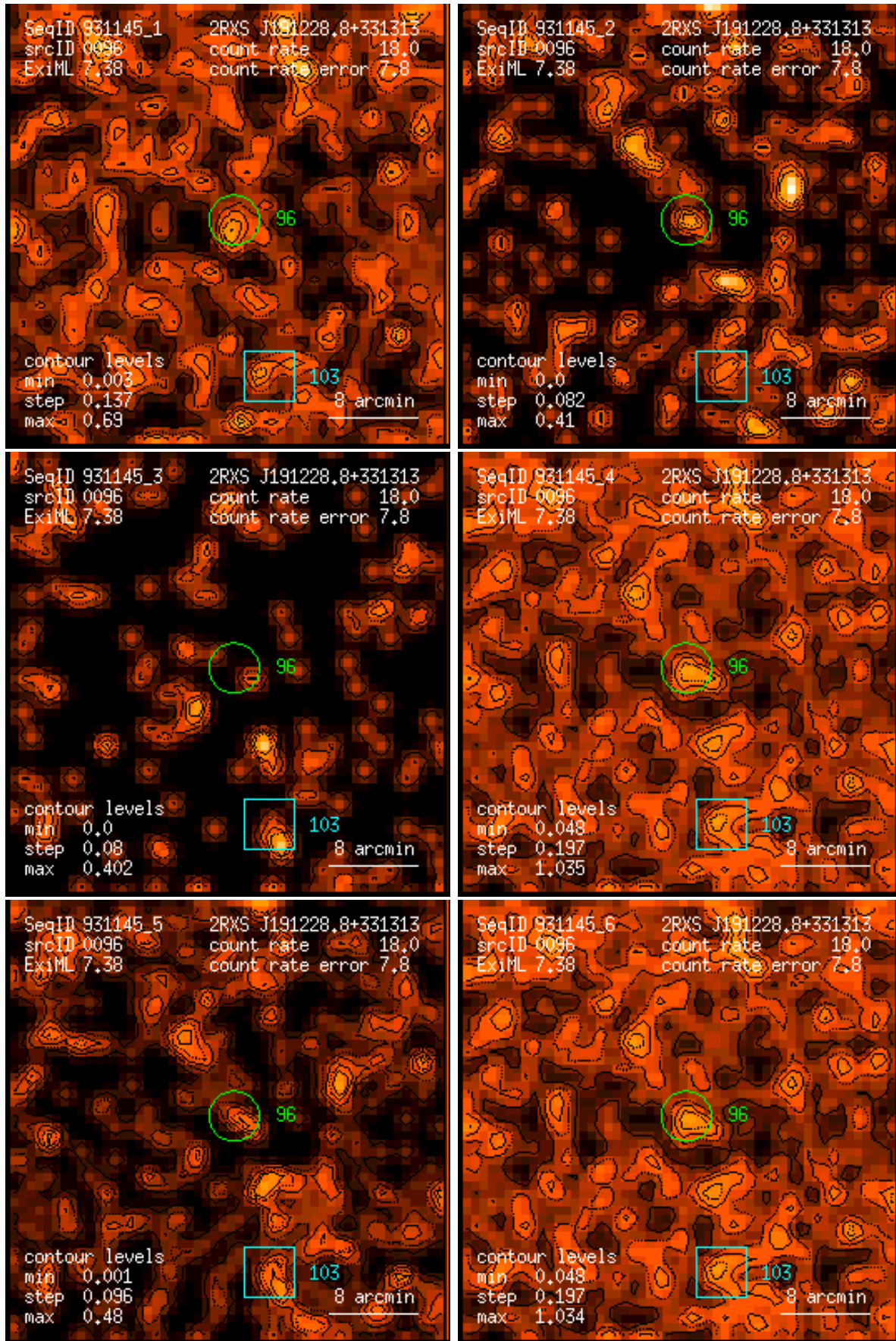
Figure 96: RASS 931145: detection 0096: band rate images, Gaussian filter: (1) PSPC channels 11 – 41, (2) 52 – 90, (3) 91 – 201, (4) 11 – 235, (5) 52 – 201, (6) 11 – 201. Broad band rates in counts/ks. Band rate contour levels in counts/ks/arcmin 2 .
