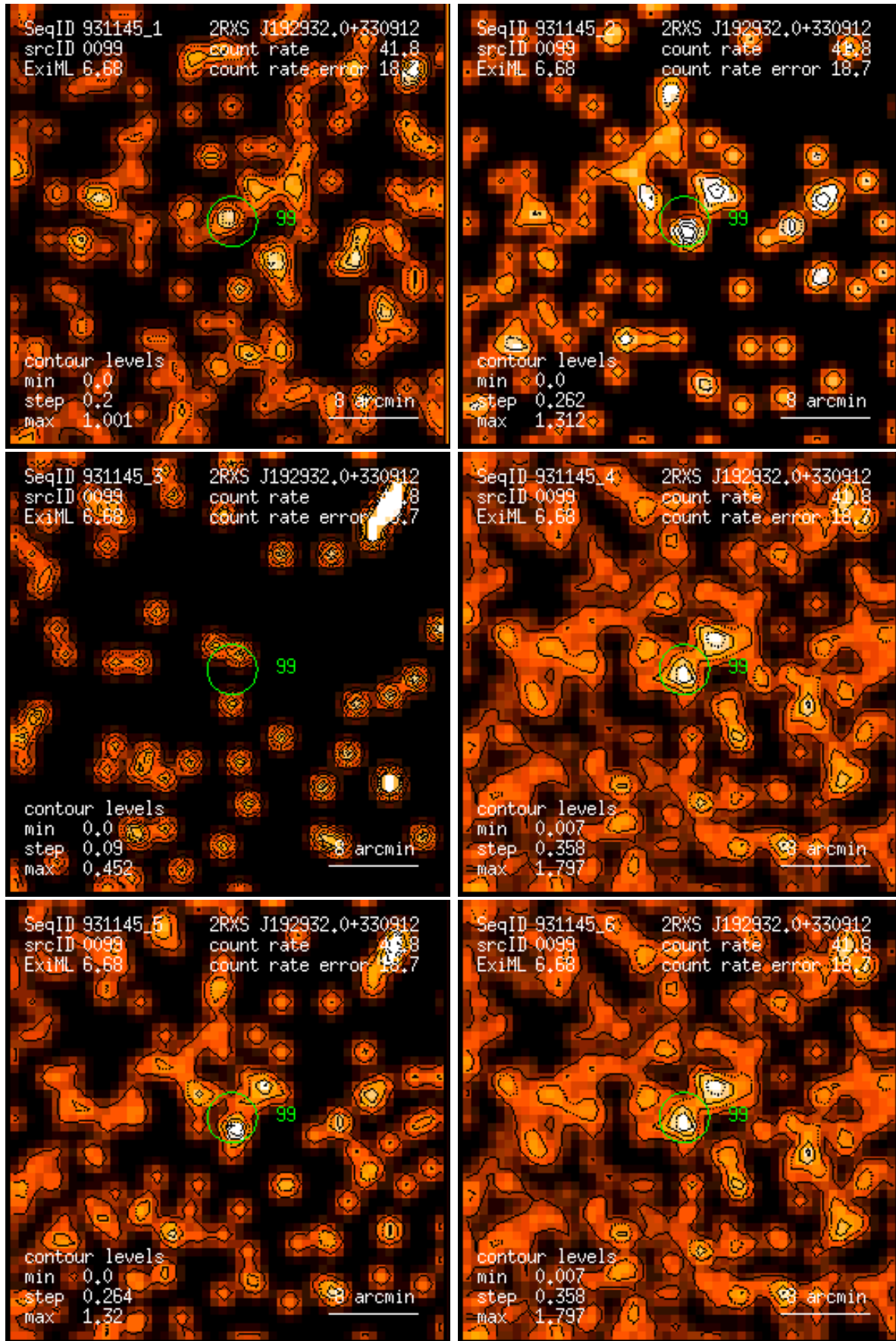
Figure 99: RASS 931145: detection 0099: band rate images, Gaussian filter: (1) PSPC channels 11 – 41, (2) 52 – 90, (3) 91 – 201, (4) 11 – 235, (5) 52 – 201, (6) 11 – 201. Broad band rates in counts/ks. Band rate contour levels in counts/ks/arcmin 2 .
