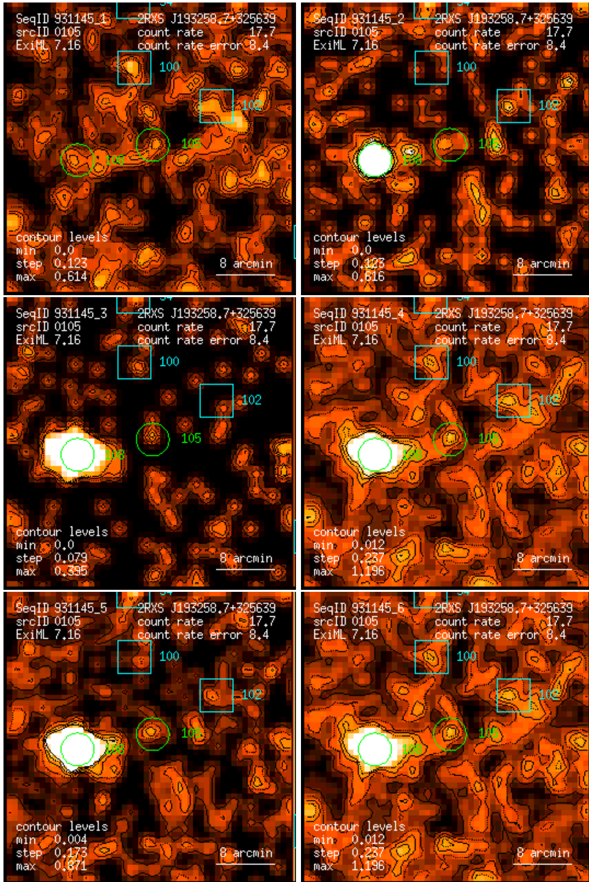
Figure 105: RASS 931145: detection 0105: band rate images, Gaussian filter: (1) PSPC channels 11 – 41, (2) 52 – 90, (3) 91 – 201, (4) 11 – 235, (5) 52 – 201, (6) 11 – 201. Broad band rates in counts/ks. Band rate contour levels in counts/ks/arcmin 2 .
