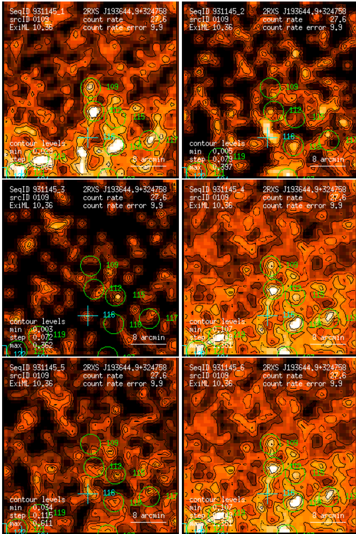
Figure 109: RASS 931145: detection 0109: band rate images, Gaussian filter: (1) PSPC channels 11 – 41, (2) 52 – 90, (3) 91 – 201, (4) 11 – 235, (5) 52 – 201, (6) 11 – 201. Broad band rates in counts/ks. Band rate contour levels in counts/ks/arcmin 2 .
