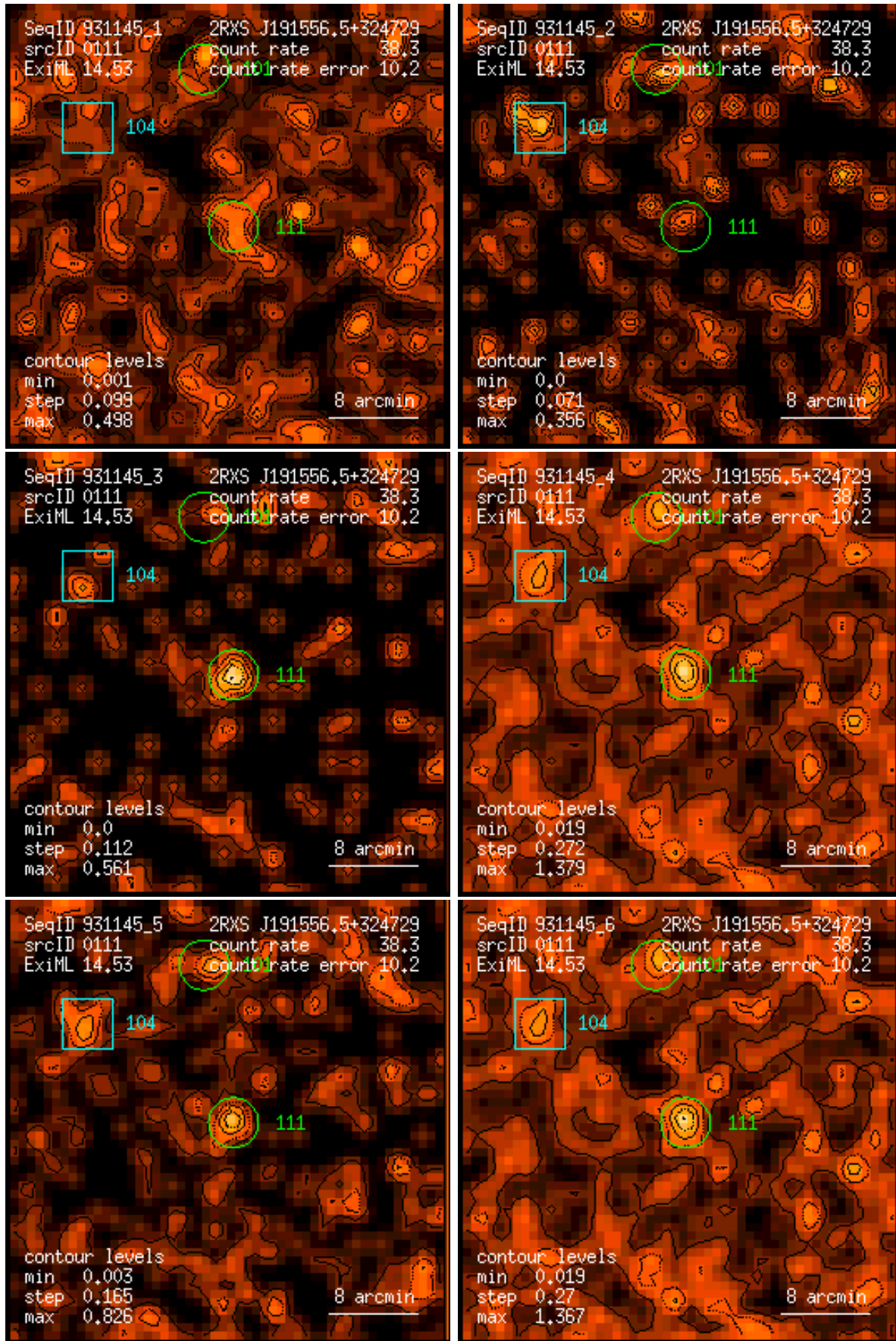
Figure 111: RASS 931145: detection 0111: band rate images, Gaussian filter: (1) PSPC channels 11 – 41, (2) 52 – 90, (3) 91 – 201, (4) 11 – 235, (5) 52 – 201, (6) 11 – 201. Broad band rates in counts/ks. Band rate contour levels in counts/ks/arcmin 2 .
