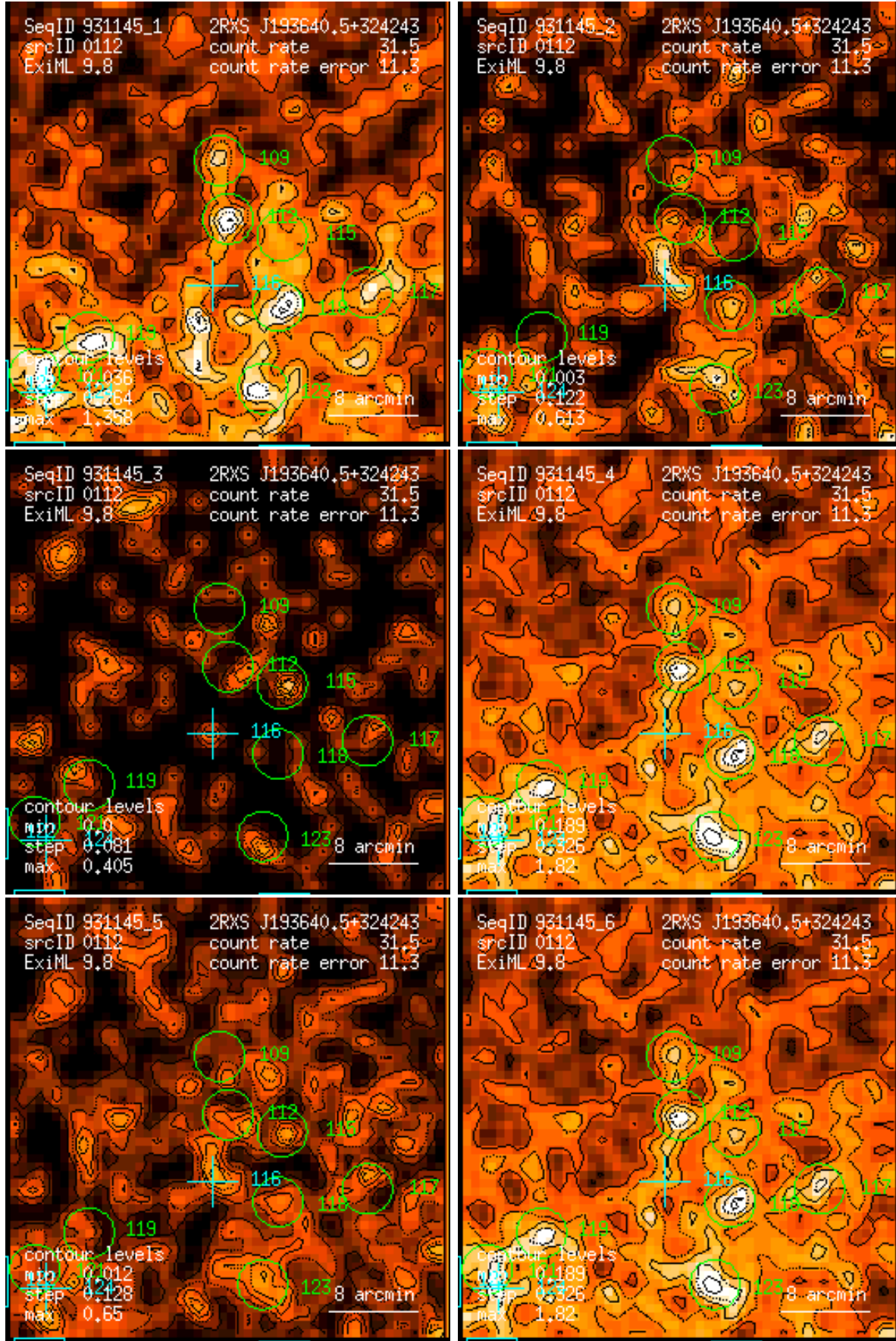
Figure 112: RASS 931145: detection 0112: band rate images, Gaussian filter: (1) PSPC channels 11 – 41, (2) 52 – 90, (3) 91 – 201, (4) 11 – 235, (5) 52 – 201, (6) 11 – 201. Broad band rates in counts/ks. Band rate contour levels in counts/ks/arcmin 2 .
