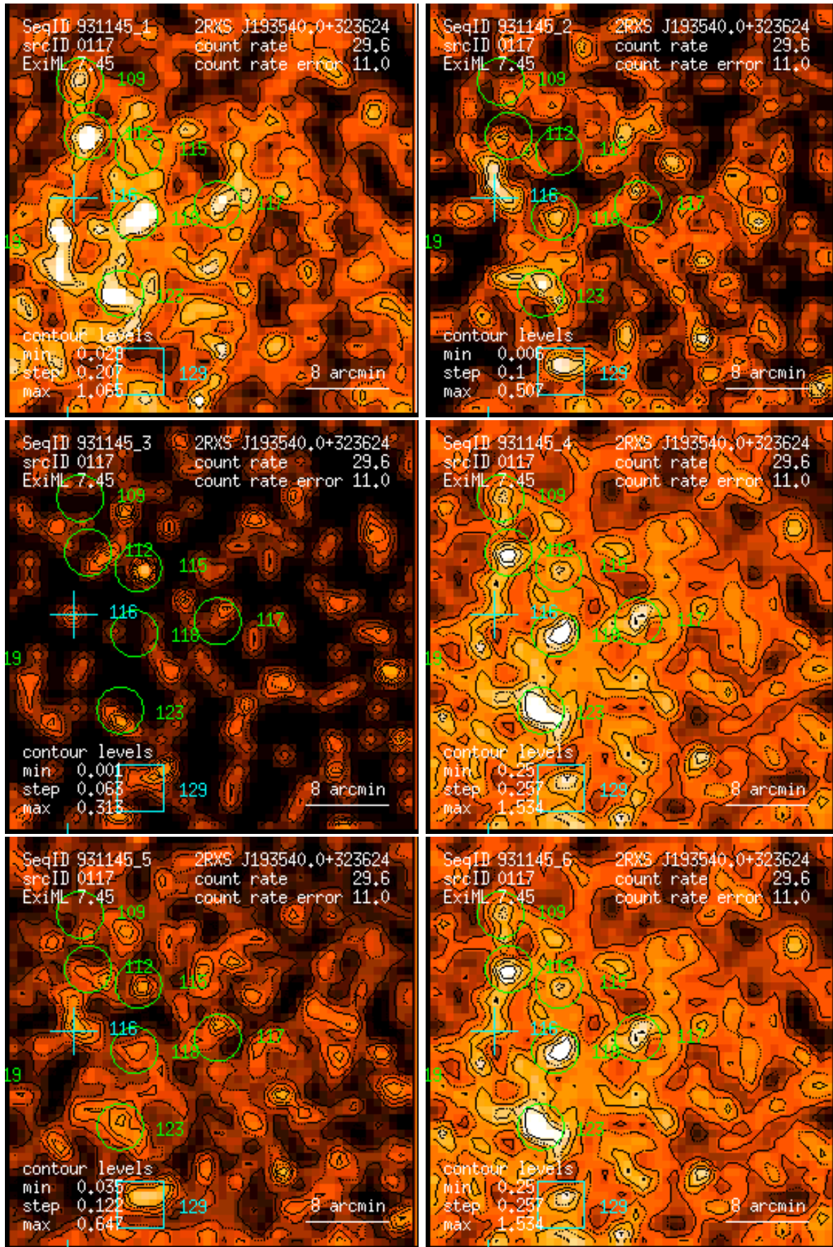
Figure 117: RASS 931145: detection 0117: band rate images, Gaussian filter: (1) PSPC channels 11 – 41, (2) 52 – 90, (3) 91 – 201, (4) 11 – 235, (5) 52 – 201, (6) 11 – 201. Broad band rates in counts/ks. Band rate contour levels in counts/ks/arcmin 2 .
