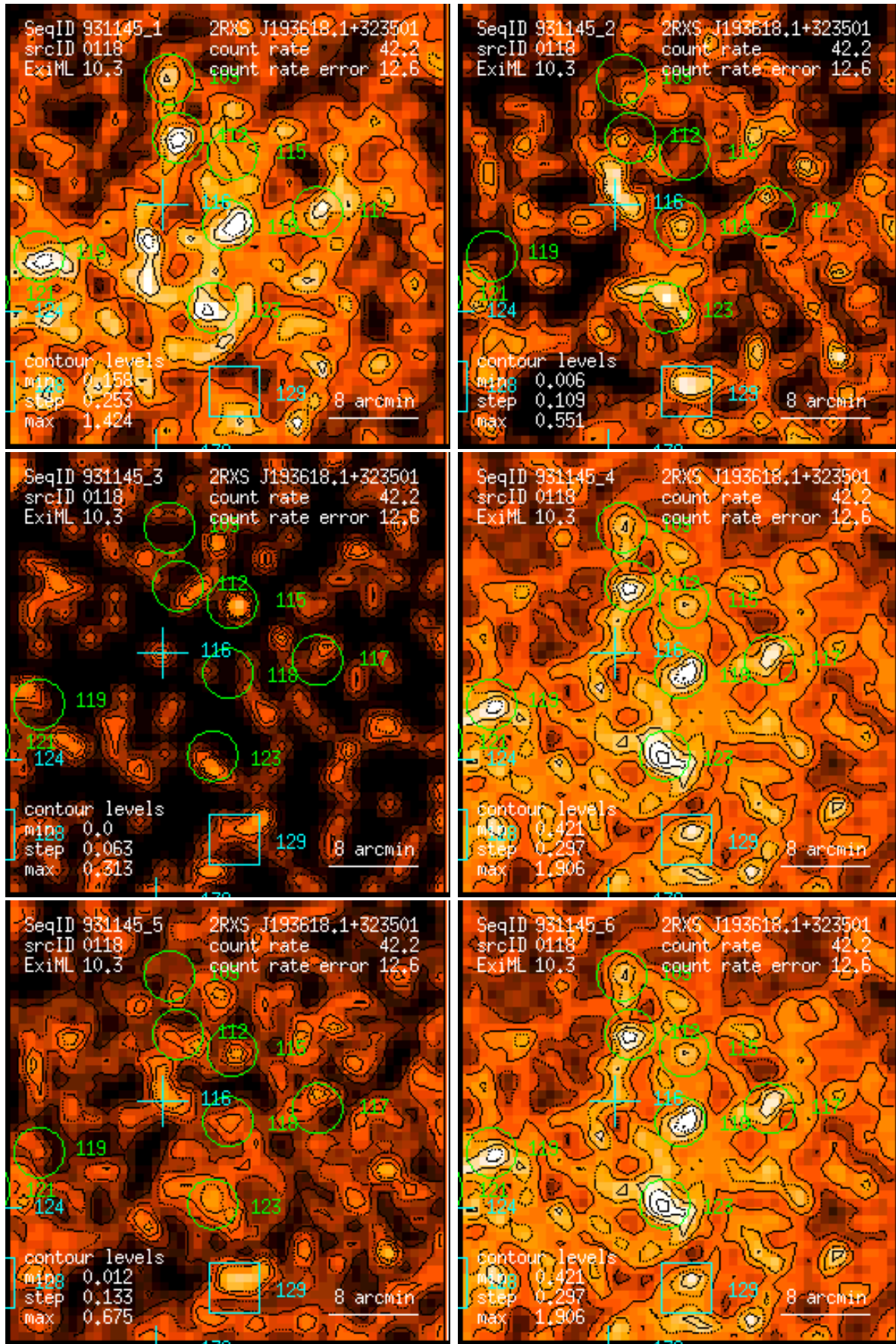
Figure 118: RASS 931145: detection 0118: band rate images, Gaussian filter: (1) PSPC channels 11 – 41, (2) 52 – 90, (3) 91 – 201, (4) 11 – 235, (5) 52 – 201, (6) 11 – 201. Broad band rates in counts/ks. Band rate contour levels in counts/ks/arcmin 2 .
