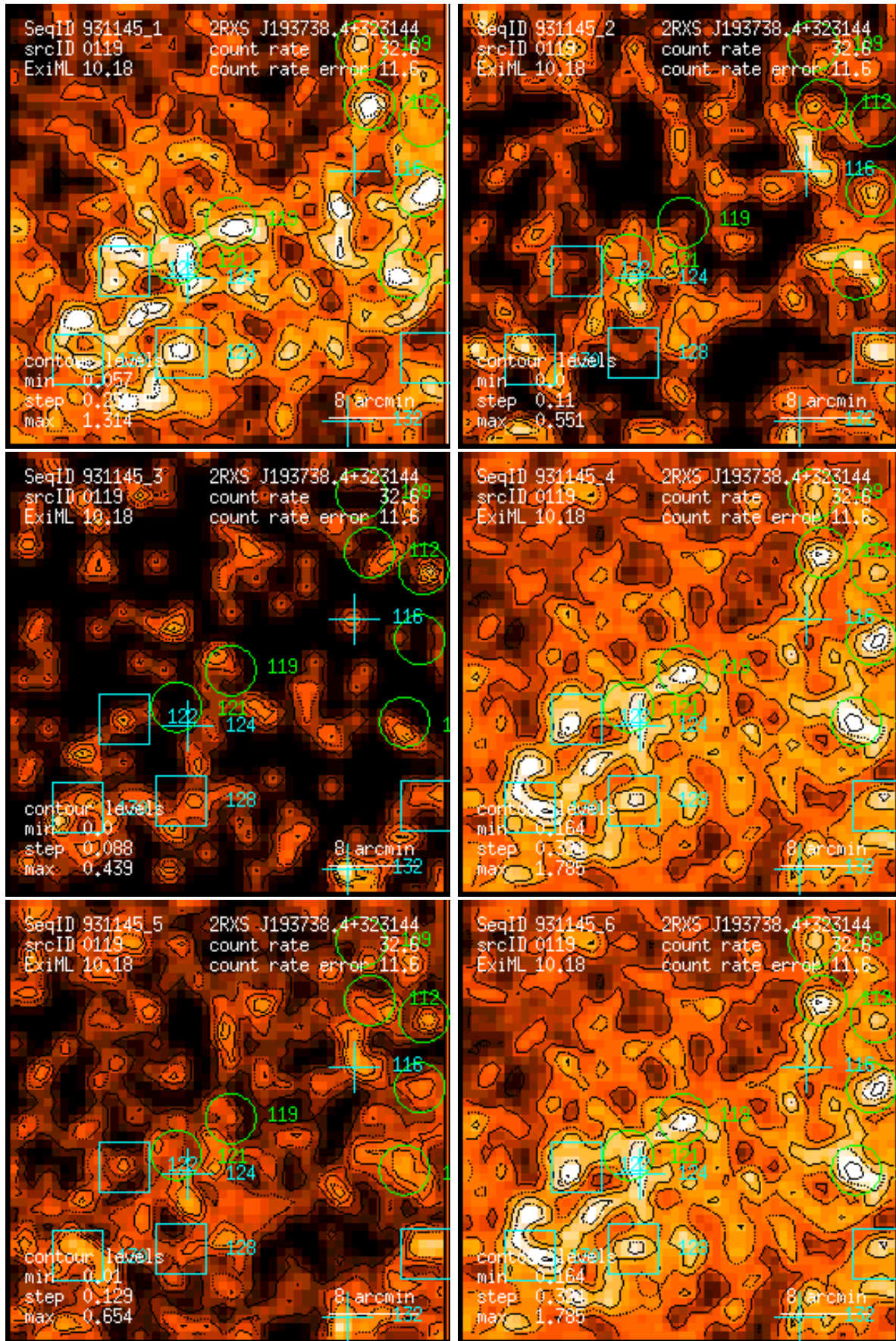
Figure 119: RASS 931145: detection 0119: band rate images, Gaussian filter: (1) PSPC channels 11 – 41, (2) 52 – 90, (3) 91 – 201, (4) 11 – 235, (5) 52 – 201, (6) 11 – 201. Broad band rates in counts/ks. Band rate contour levels in counts/ks/arcmin 2 .
