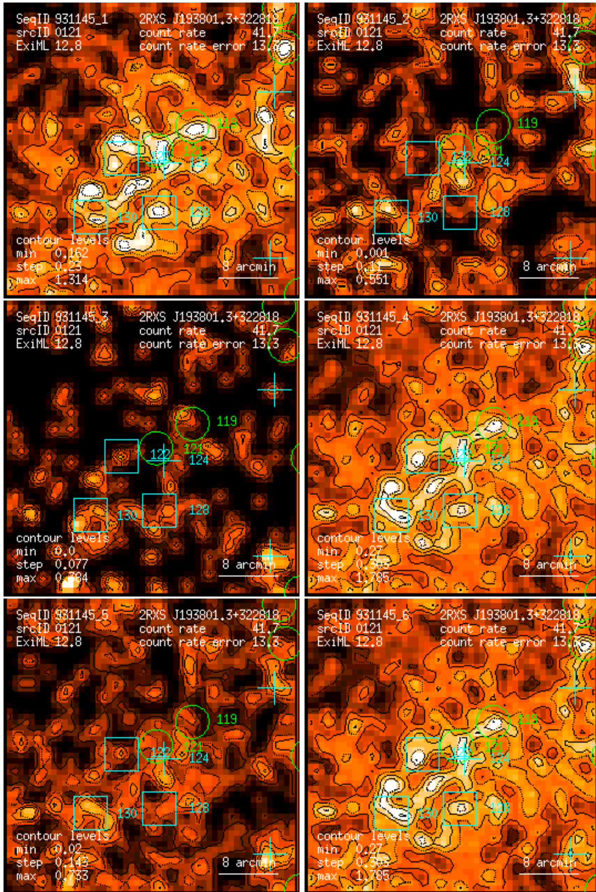
Figure 121: RASS 931145: detection 0121: band rate images, Gaussian filter: (1) PSPC channels 11 – 41, (2) 52 – 90, (3) 91 – 201, (4) 11 – 235, (5) 52 – 201, (6) 11 – 201. Broad band rates in counts/ks. Band rate contour levels in counts/ks/arcmin 2 .
