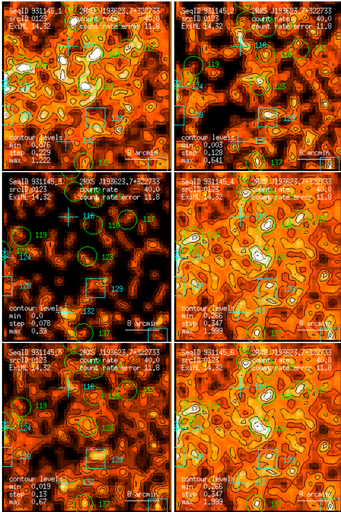
Figure 123: RASS 931145: detection 0123: band rate images, Gaussian filter: (1) PSPC channels 11 – 41, (2) 52 – 90, (3) 91 – 201, (4) 11 – 235, (5) 52 – 201, (6) 11 – 201. Broad band rates in counts/ks. Band rate contour levels in counts/ks/arcmin 2 .
