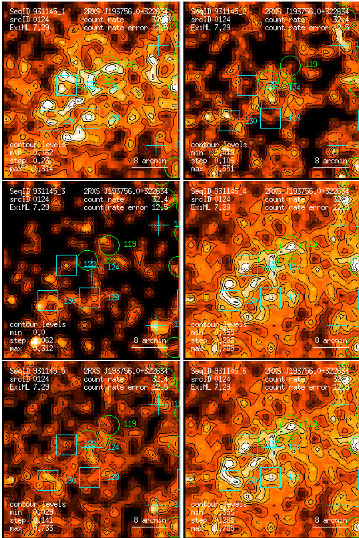
Figure 124: RASS 931145: detection 0124: band rate images, Gaussian filter: (1) PSPC channels 11 – 41, (2) 52 – 90, (3) 91 – 201, (4) 11 – 235, (5) 52 – 201, (6) 11 – 201. Broad band rates in counts/ks. Band rate contour levels in counts/ks/arcmin 2 .
