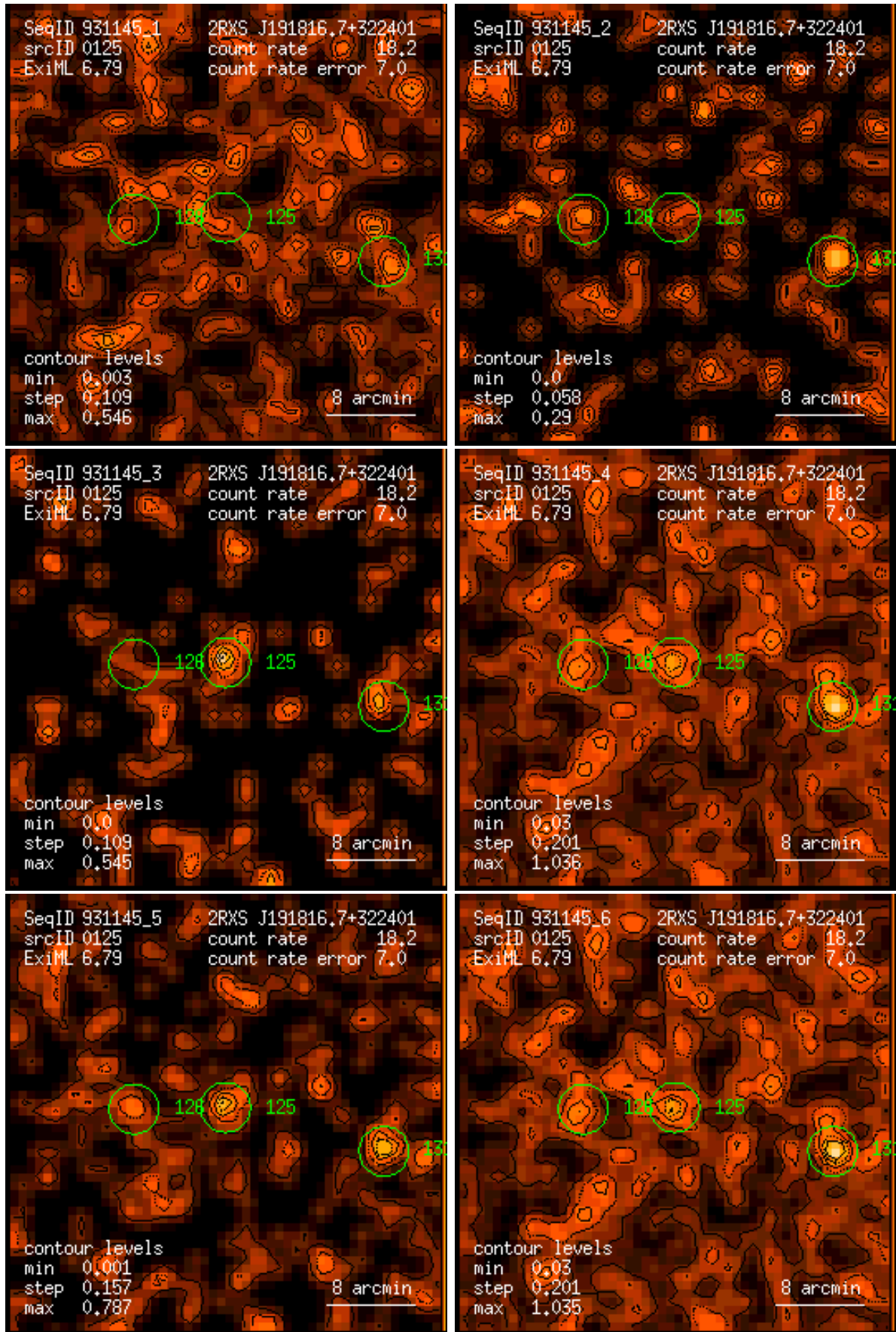
Figure 125: RASS 931145: detection 0125: band rate images, Gaussian filter: (1) PSPC channels 11 – 41, (2) 52 – 90, (3) 91 – 201, (4) 11 – 235, (5) 52 – 201, (6) 11 – 201. Broad band rates in counts/ks. Band rate contour levels in counts/ks/arcmin 2 .
