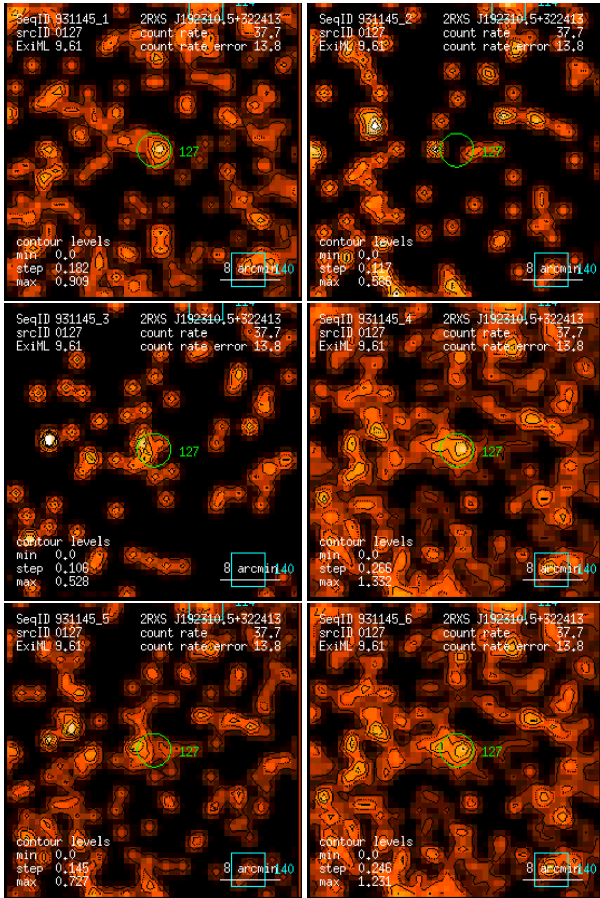
Figure 127: RASS 931145: detection 0127: band rate images, Gaussian filter: (1) PSPC channels 11 – 41, (2) 52 – 90, (3) 91 – 201, (4) 11 – 235, (5) 52 – 201, (6) 11 – 201. Broad band rates in counts/ks. Band rate contour levels in counts/ks/arcmin 2 .
