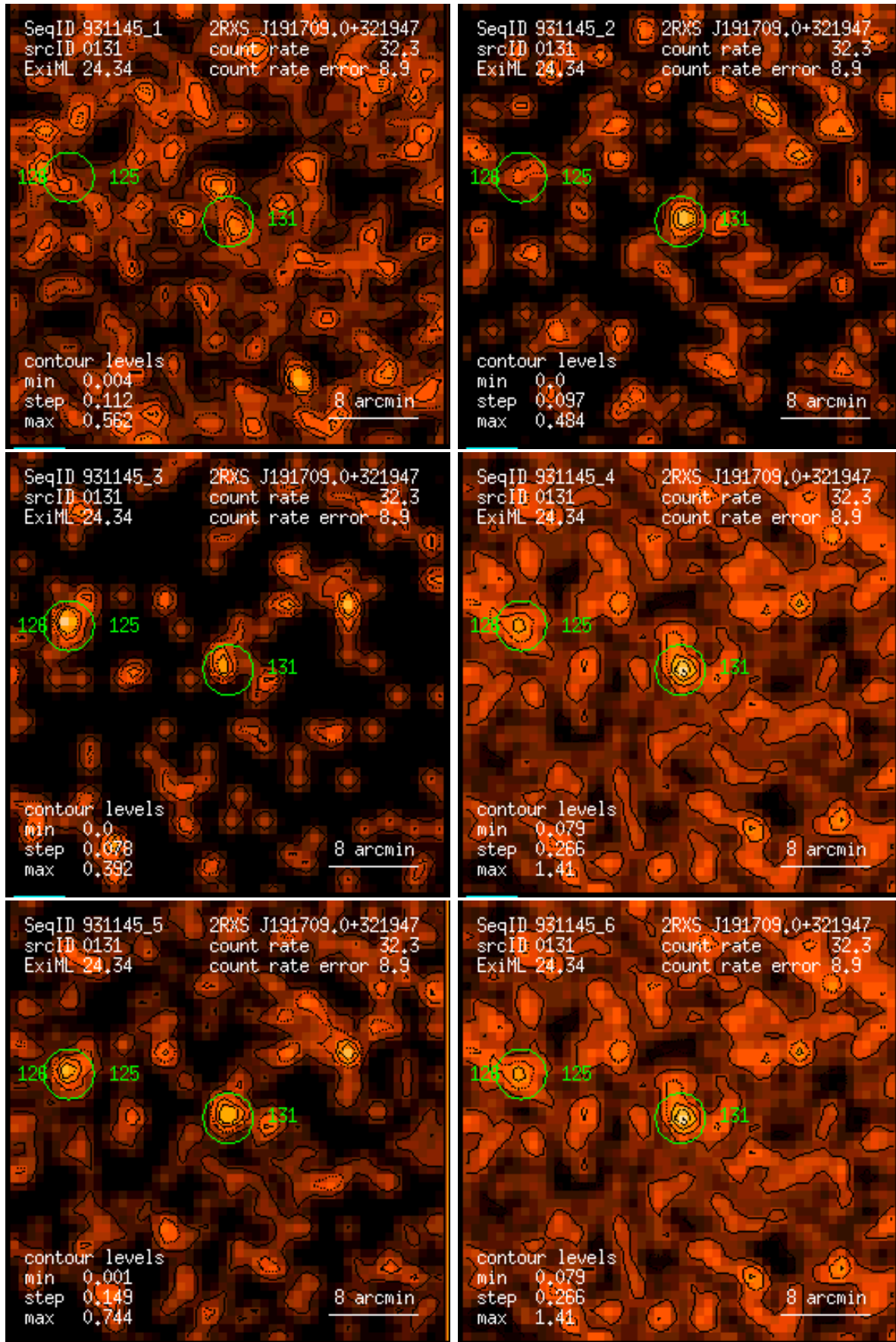
Figure 131: RASS 931145: detection 0131: band rate images, Gaussian filter: (1) PSPC channels 11 – 41, (2) 52 – 90, (3) 91 – 201, (4) 11 – 235, (5) 52 – 201, (6) 11 – 201. Broad band rates in counts/ks. Band rate contour levels in counts/ks/arcmin 2 .
