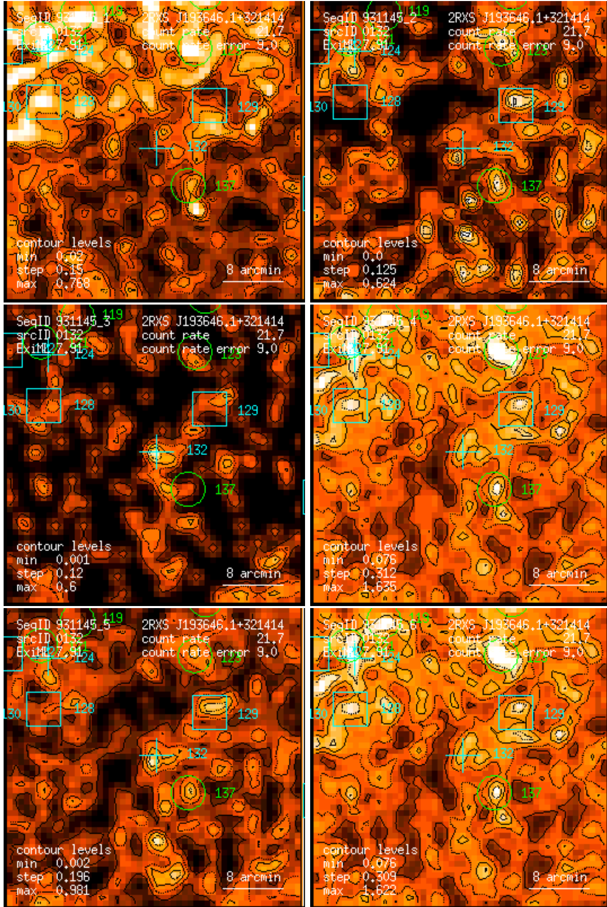
Figure 132: RASS 931145: detection 0132: band rate images, Gaussian filter: (1) PSPC channels 11 – 41, (2) 52 – 90, (3) 91 – 201, (4) 11 – 235, (5) 52 – 201, (6) 11 – 201. Broad band rates in counts/ks. Band rate contour levels in counts/ks/arcmin 2 .
