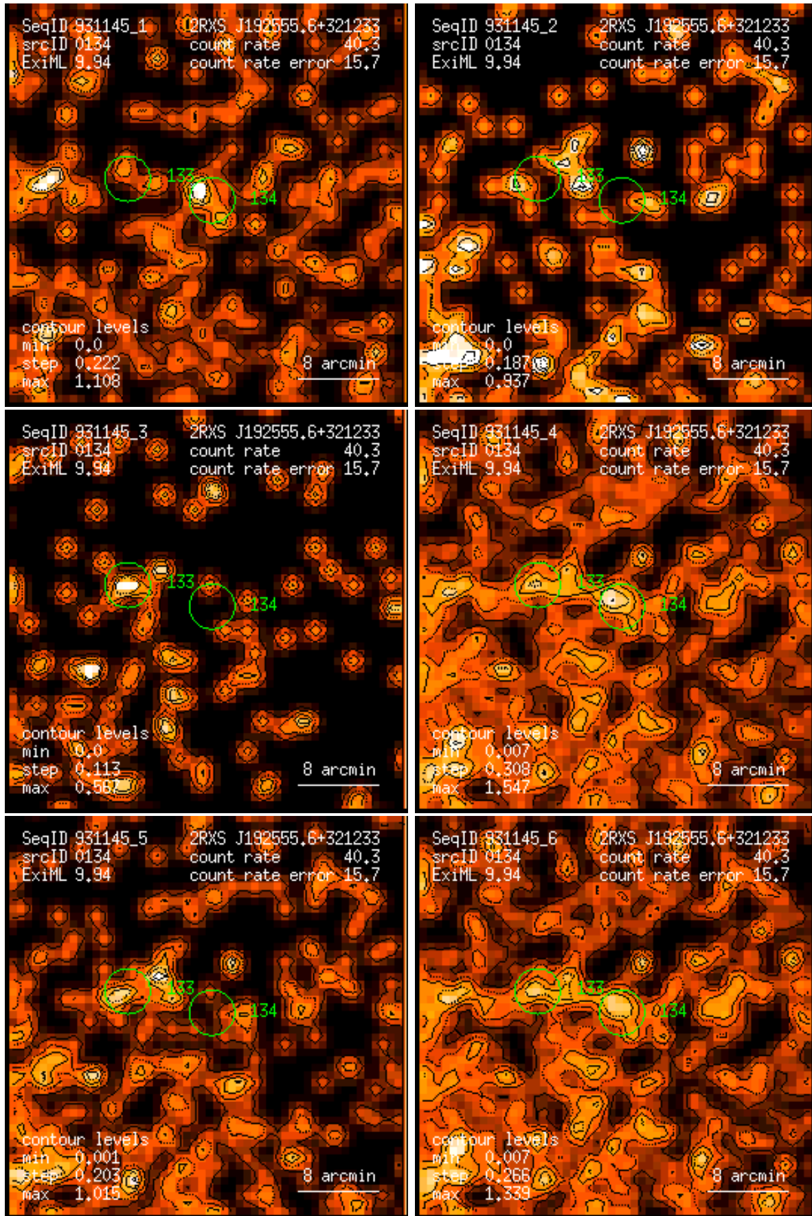
Figure 134: RASS 931145: detection 0134: band rate images, Gaussian filter: (1) PSPC channels 11 – 41, (2) 52 – 90, (3) 91 – 201, (4) 11 – 235, (5) 52 – 201, (6) 11 – 201. Broad band rates in counts/ks. Band rate contour levels in counts/ks/arcmin 2 .
