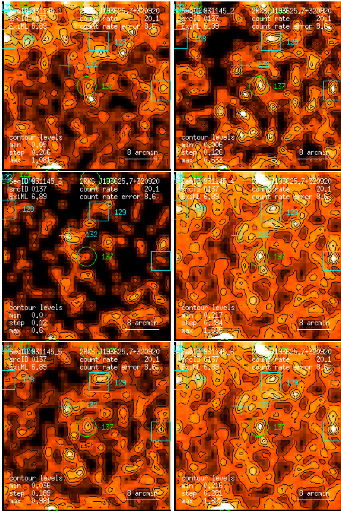
Figure 137: RASS 931145: detection 0137: band rate images, Gaussian filter: (1) PSPC channels 11 – 41, (2) 52 – 90, (3) 91 – 201, (4) 11 – 235, (5) 52 – 201, (6) 11 – 201. Broad band rates in counts/ks. Band rate contour levels in counts/ks/arcmin 2 .
